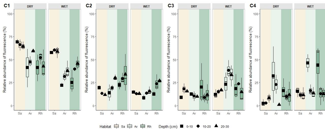
660 Figure A7: EEM contour plots of the four PARAFAC components (C1, C2, C3, C4) and seasonal variations in their relative fluorescence abundance (%) across a land-sea gradient in (salt-flat (Sa), Avicennia marina (Av), and Rhizophora stylosa (Rh)). Symbols represent soil depth layers (squares: 0-10 cm; circles: 10-20 cm; triangles: 20-30 cm).
