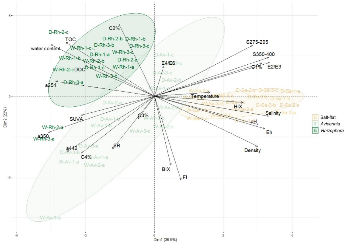
Figure 2 : Biplot of principal component analysis (PCA) (Dim 1: 39.9%, Dim 2: 22%) with K-means Clustering (K = 3). Absorption coefficients a 254 , a 350 , and a 442 correspond to CDOM absorption (m -1 ) at 254, 350, and 442 nm, respectively. Sample codes follow the structure Season-Habitat-Core replicate-Depth (e.g., W-Sa-1-a corresponds to Wet season, Salt-flat, core 1, surface layer).
