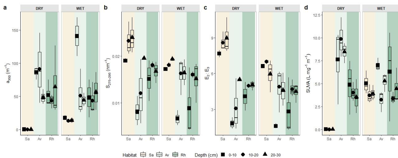
Figure A6: Seasonal and spatial variations of CDOM indicators ( a_{350} [a], S_{275-295} [b], E_2/E_3 [c], and SUVA [d]) across a land-sea gradient in salt-flat (Sa), Avicennia marina (Av), and Rhizophora stylosa (Rh). Symbols represent soil depth layers (squares: 0-10 cm; circles: 10-20 cm; triangles: 20-30 cm).
