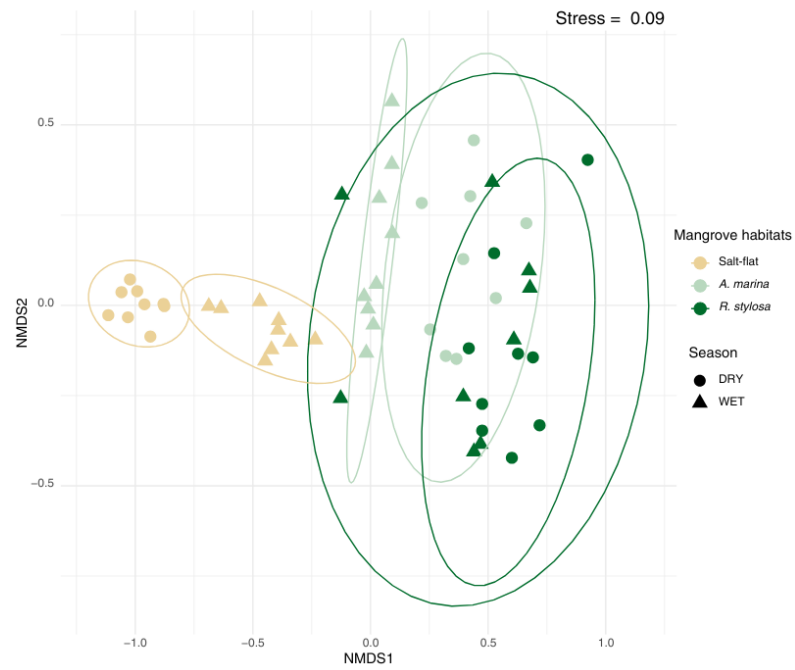
640 Figure A3: Non metric multidimensional scaling (nMDS) ordination of sampling units based on Bray-Curtis dissimilarities of standardized environmental variables in a total of N = 54 sampling units (n = 3 replicates from each of the three mangrove habitat at 3 depths during 2 seasons) in the Bouraké mangrove ecosystem. Colours indicate the mangroves habitat; ellipse represent clusters and symbols show seasons.
