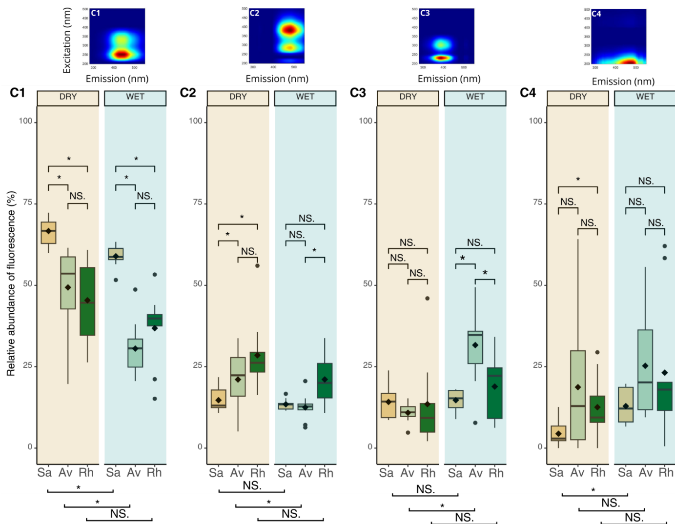
375 Figure 7 : EEM contour plots of the four PARAFAC components (C1, C2, C3, C4) and seasonal variations in their relative fluorescence abundance (%) across a land-sea gradient in (salt-flat (Sa), Avicennia marina (Av), and Rhizophora stylosa (Rh)). Significant differences between habitats (ANOVA/Kruskal-Wallis, see Table A8 for full test results) and between seasons (Student's t-test/Mann-Whitney) are indicated (* p < 0.05 , NS = no significant difference, see Table A7 for full test results). Variations across soil depth layers are presented in Fig. A7.
