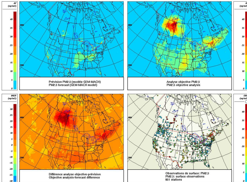
Figure 4. Four-panel presentation of RDAQA 2.0.0 results for PM_{2.5} surface concentration ( \mu g m^{-3} ) for 28 Sept. 2023 at 16 UTC: (a) RAQDPS023 PM_{2.5} forecast; (b) RDAQA 2.0.0 PM_{2.5} objective analysis; (c) PM_{2.5} analysis increment (correction to the model forecast); and (d) PM_{2.5} surface observations.
