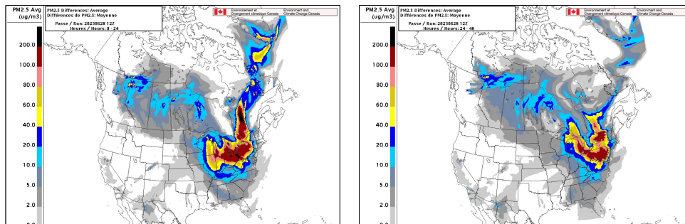
Figure 5. RAQDPS-FW 12 UTC forecast on 28 June 2023 of contribution of smoke from wildfires to mean surface PM_{2.5} concentrations ( \mu g m^{-3} ) for hours (a) 00-24 and (b) 24-48.
