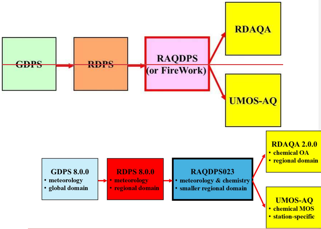
3420 Figure 1. Current RAQDPS023 “upstream” and “downstream” dependencies on other ECCC operational systems.
