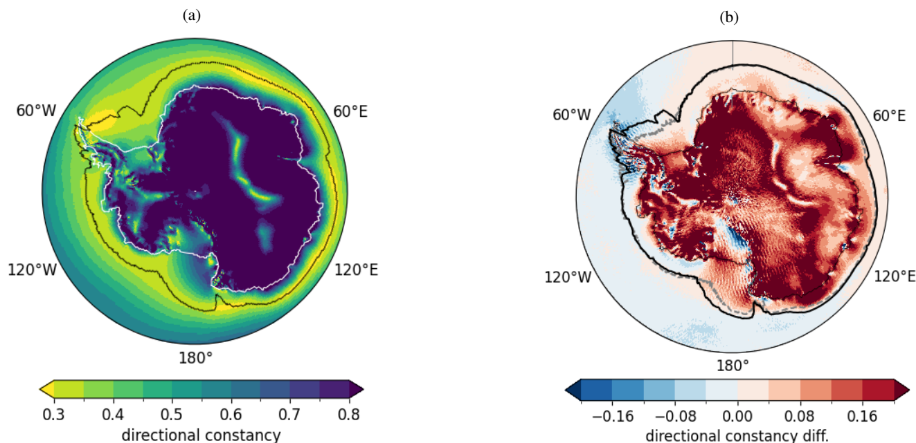
Figure 2. (a) The time-averaged directional constancy across the Antarctic region (60S–90S) from 1980–2023 using ERA5 wind data. Black contour indicates the time-averaged ACWB. (b) Also using ERA5 wind data, the actual minus large-scale directional constancy, time-averaged from 2010–2020 (Caton Harrison et al., 2024). Black contour shows the time-averaged ACWB; grey, dashed line shows the ACWB for the calculated large-scale wind field.
