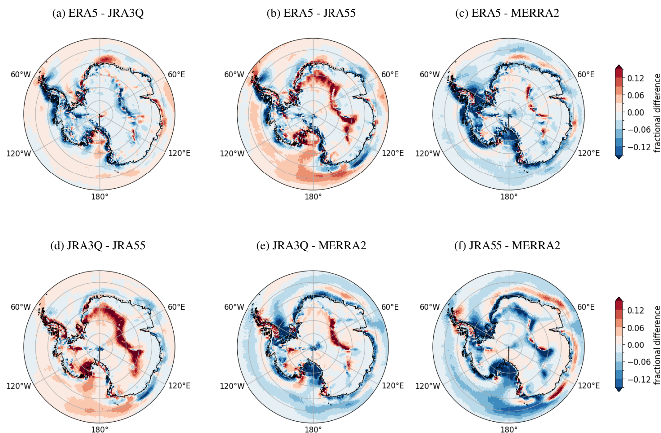
Figure A1. The fractional difference of the mean directional constancy, calculated from monthly wind data, between the 4 reanalysis products. Fractional difference calculated, for example, between ERA5 & JRA3Q as \frac{2(ERA5 - JRA3Q)}{ERA5 + JRA3Q} .
