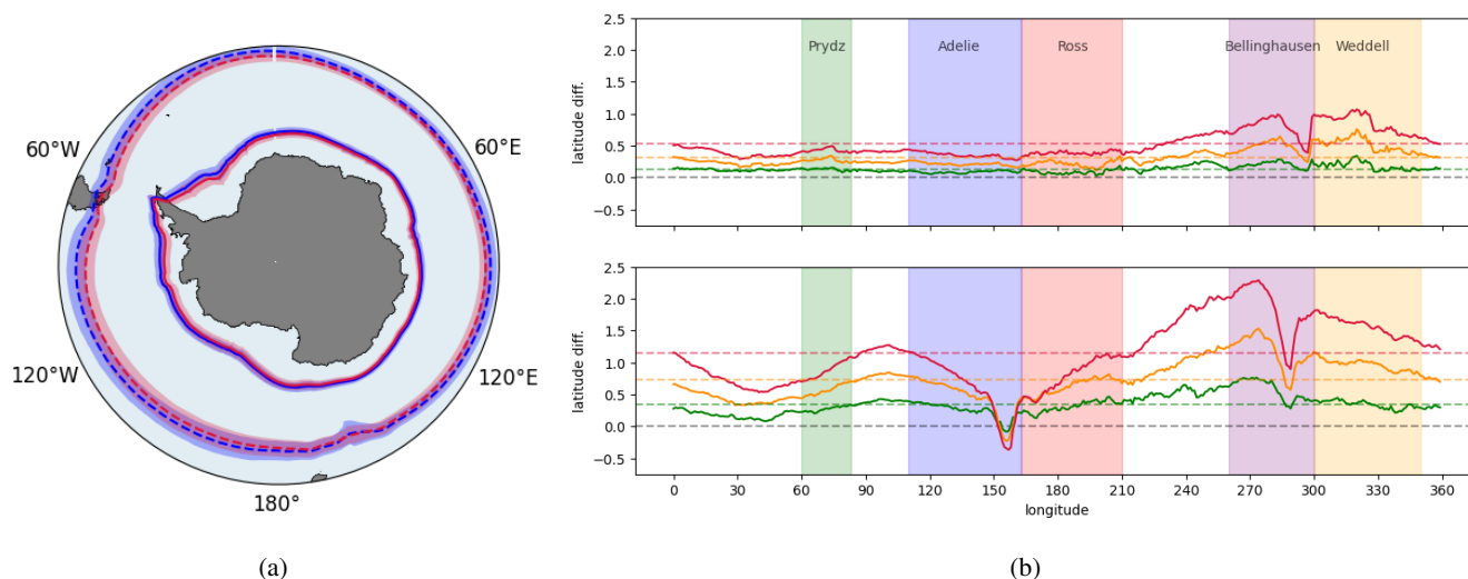
Figure 7. (a) The time-averaged JLI (dashed) and ACWB (solid) for the multi-model means of CMIP6, 2020–2039 (blue) and CMIP6, 2080–2099 (red). The shaded regions are the \pm 1 standard deviation of the CMIP6 models. (b) The difference between the 2020–2039 and 2080–2099 (red, upper), 2060–2079 (orange, middle), 2040–2059 (green, lower) models for the JLI (bottom plot) and ACWB (top plot). The dashed, coloured lines are the mean difference over latitude, while the grey dashed line is zero.
