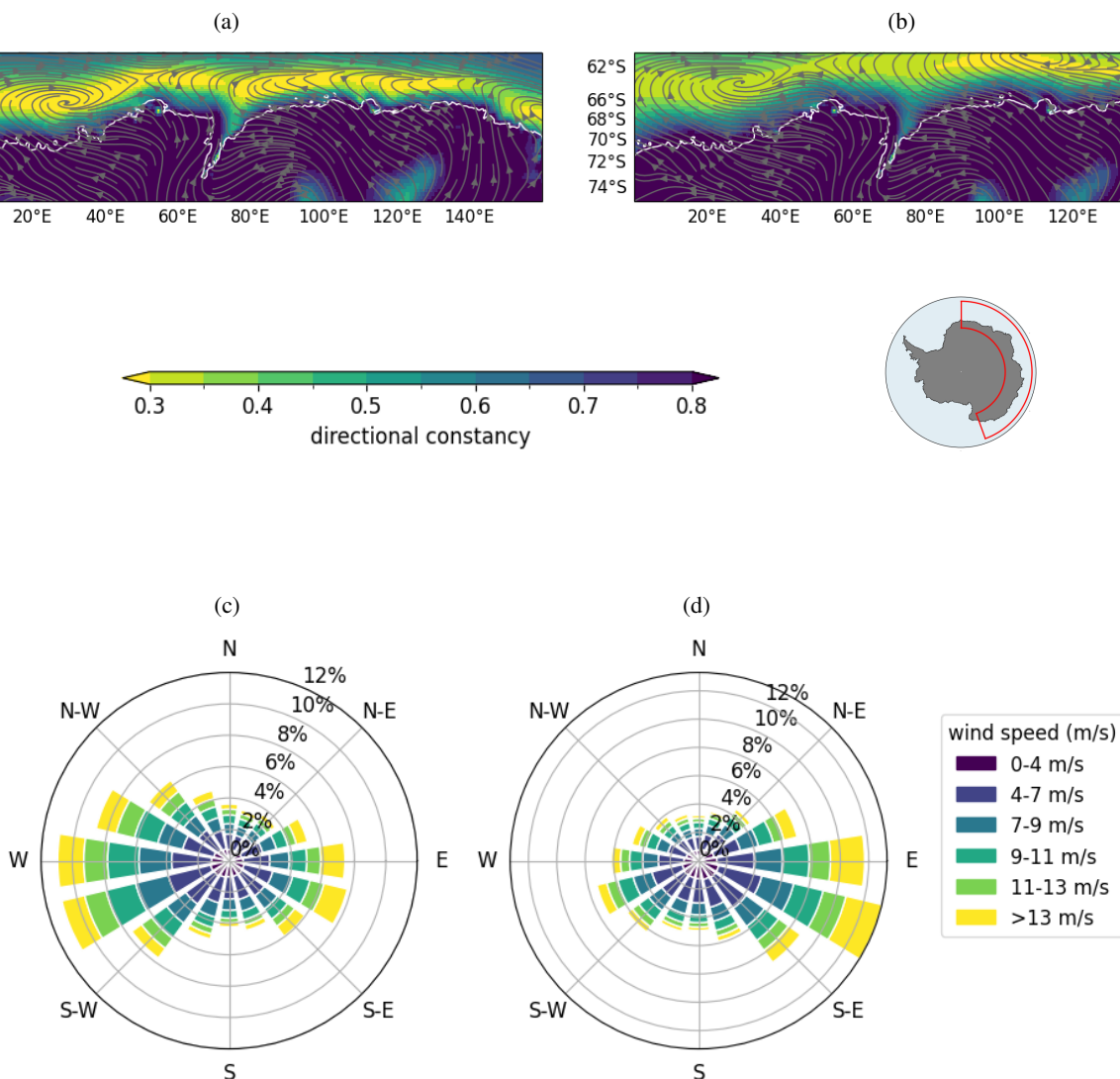
Figure 3. Directional constancy averaged over dates in the top (a) and bottom (b) 10% values in the leading principal component timeseries, using monthly ERA5 wind data in the East Antarctic region (red, boxed region on right map: 0-160E, 60S-90S). Grey arrows indicate the monthly winds averaged over the same dates. (c) & (d) are the wind rose plots, based on 6-hourly wind data over the ocean, associated with (a) and (b) respectively.
