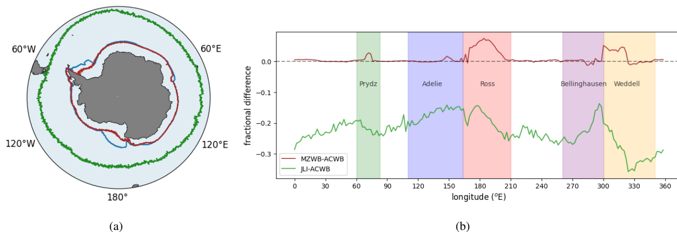
Figure 5. (a) A contour map of Antarctica with the time-averaged ACWB (blue), MZWB (red, inner) and JLI (green, outer) from ERA5 10 m wind data and (b) the difference between the MZWB and ACWB (red, upper) and between the JLI and ACWB (green, lower), smoothed by 2^\circ over longitude. The boxes contain the correlation over longitude between the time-averaged MZWB and ACWB (red, upper) and JLI and ACWB (green, lower). Grey dashed line in (b) is zero fractional difference.
