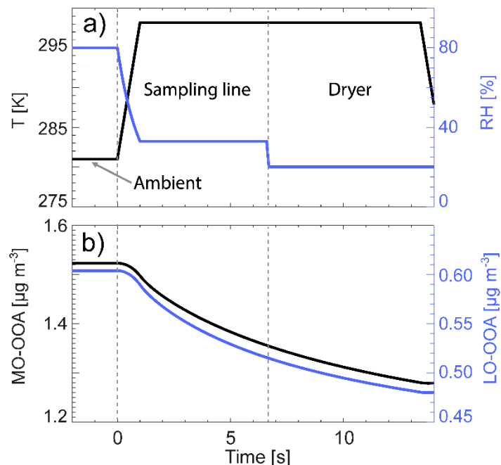
Figure 4. Time series of a) RH and temperature and b) the condensed mass concentration of MO-OOA and LO-OOA in the sampling line and the dryer for VBS 1. The mass concentration at 14 s corresponds to the measured, and the one at 0 s to the estimated ambient mass concentration.
