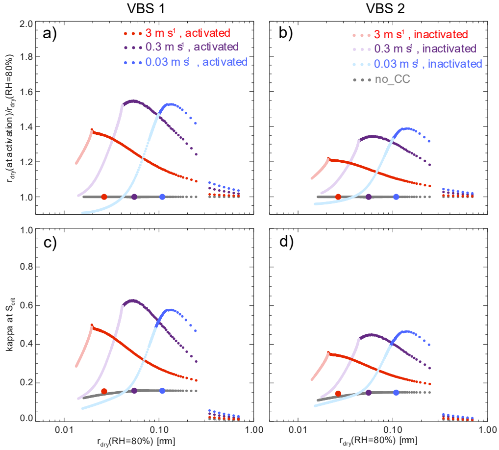
Figure 8. Dependence of relative dry radius (a, b) and equivalent \kappa (c, d) at the activation point on initial particle size r_{\text{dry}}(\text{RH} = 80 \%) for VBS 1 (a, c) and VBS 2 (b, d), for combined inorganic and organic co-condensation (coloured lines, co-condensation activated). The light portions of the lines represent non-activated particles evaluated at the time the last aerosol particle has activated. The grey line represents the control case without co-condensation for the updraft of 0.3 \text{ m s}^{-1} . Coloured dots on the grey line mark the smallest activated dry radii of the control cases for the different updrafts.
