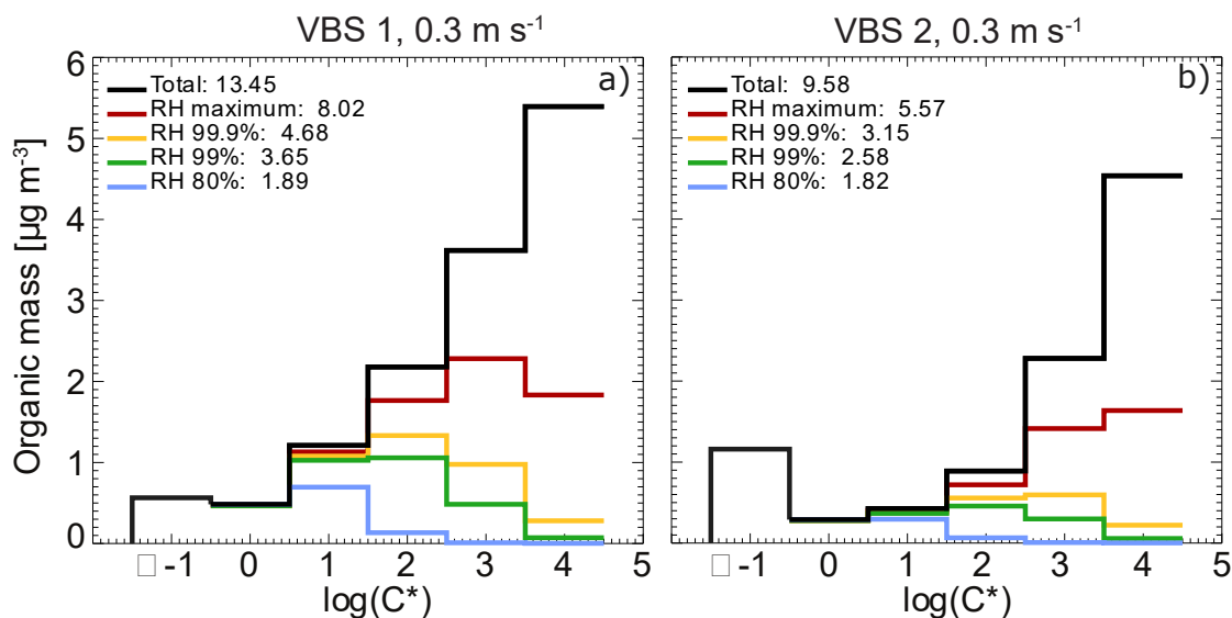
Figure 5. Total organic mass (gas and condensed phase: black line) and organic mass in the condensed phase at selected RH (coloured lines), summed up (masses given in the legend), and per volatility bins in the VBS derived in this study based on a) Tsimplidi et al. (2010) (VBS 1) and b) Cappa and Jimenez (2010) (VBS 2).
