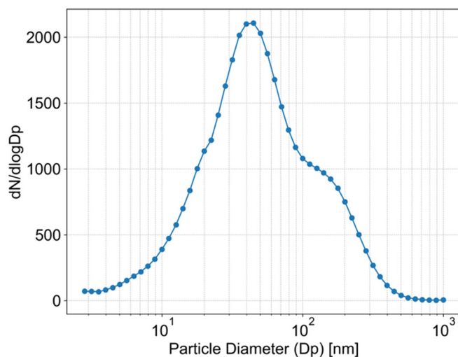
Figure 1. Campaign-averaged particle size distribution during September-November 2018. The total number of particles with diameters from 2.82 nm to 1000 nm is 1871 cm -3 .
