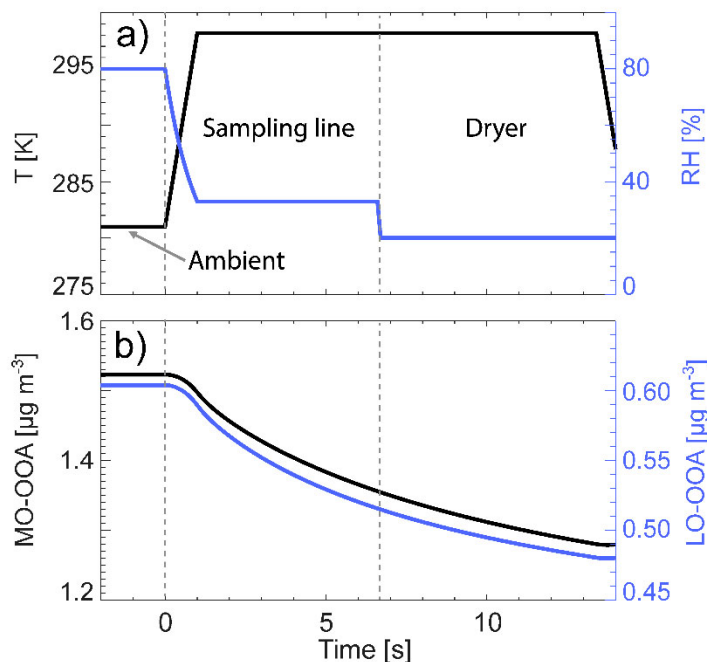
270 Figure 4. Time series of a) RH and temperature and b) the condensed mass concentration of MO-OOA and LO-OOA in the sampling line and the dryer. The mass concentration at 14 s corresponds to the measured, and the one at 0 s to the estimated ambient mass concentration.
