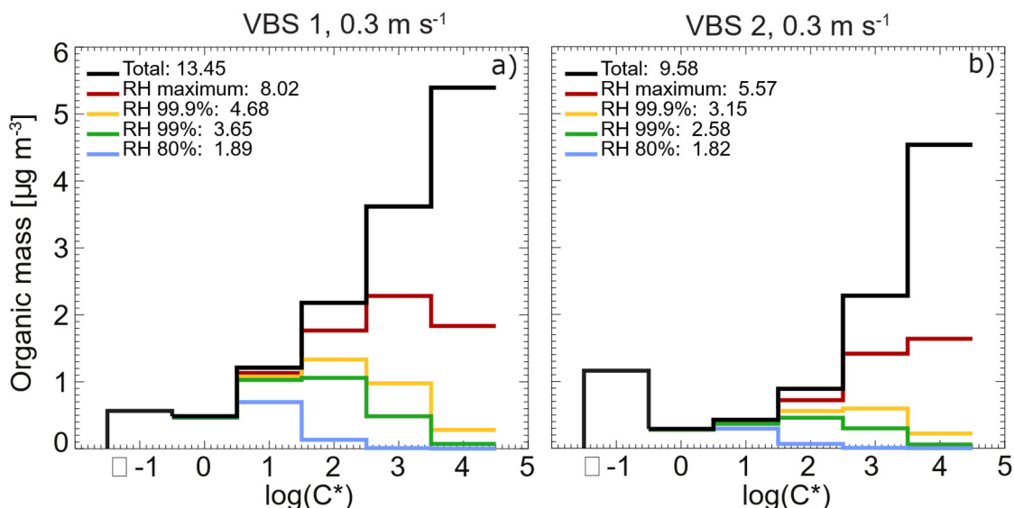
310 Figure 5. Total organic mass (gas and condensed phase: black line) and organic mass in the condensed phase at selected RH (coloured lines) summed up (masses given in the legend) and per volatility bins in the VBS derived in this study based on a) Tsimpidi et al. (2010) (VBS 1) and b) Cappa and Jimenez (2010) (VBS 2).
