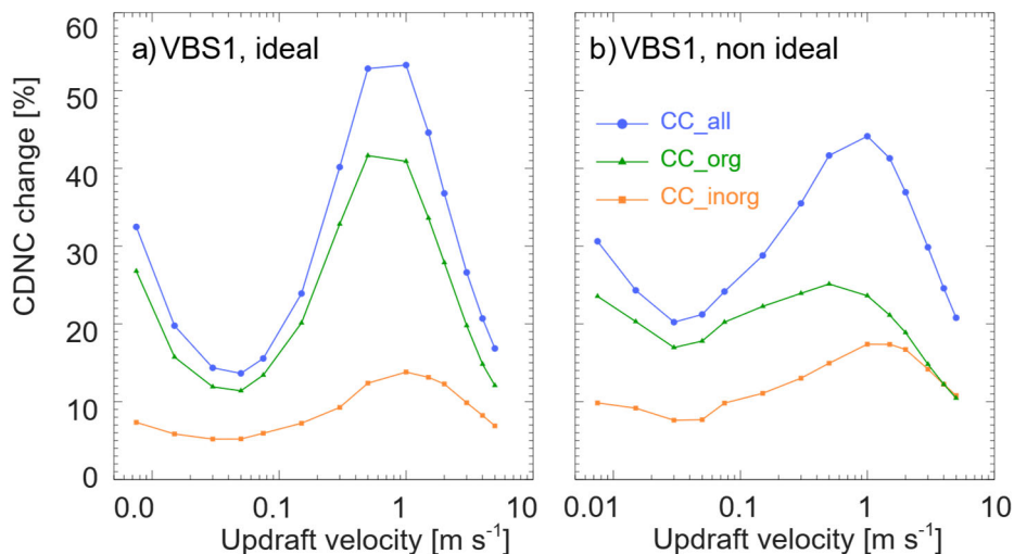
460 Figure 9. Change of CDNC as a function of updraft velocity for VBS 1, assuming solution ideality (panel a) and non-ideality (panel b) of inorganic-organic aqueous mixtures.
