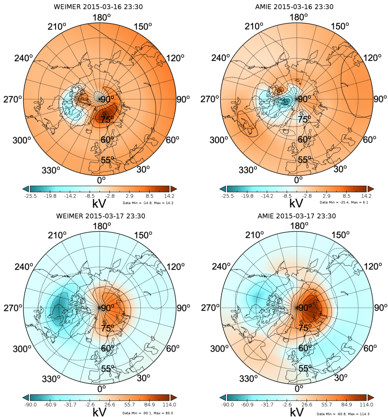
Figure 6. Electric potential maps: Upper-left: Weimer at baseline, Upper-right: AMIE at baseline, Lower-left: Weimer at peak, Lower-right: AMIE at peak
