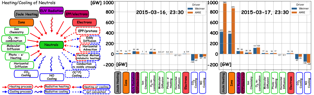
Figure 3. Left: Overview of the main energy sources and energy flow to and from the neutrals in the Lower Thermosphere - Ionosphere. Terms in solid arrows and boxes are estimated through TIE-GCM, whereas terms in dashed arrows and boxes are not calculated. Right (Middle): Quantification of the main energy terms at the peak of (one day before the peak of) St. Patrick's day storm. Two electric potential drivers are used, according to the Weimer 2005 and the AMIE models, as marked.
