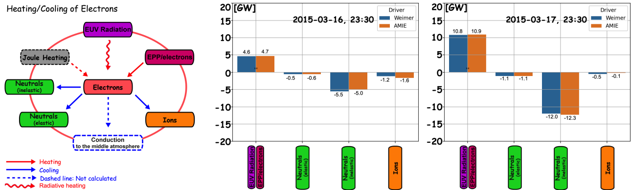
Figure 5. Left: Overview of the main energy sources and energy flow to and from the Electrons in the Lower Thermosphere - Ionosphere. Terms with red arrows correspond to heating of the electrons whereas terms with blue arrows correspond to cooling of the electrons. Right (Middle): Quantification of the main energy terms at the peak of (one day before the peak of) St. Patrick's day storm. Two electric potential drivers are used, according to the models by Weimer, and AMIE, as marked.
