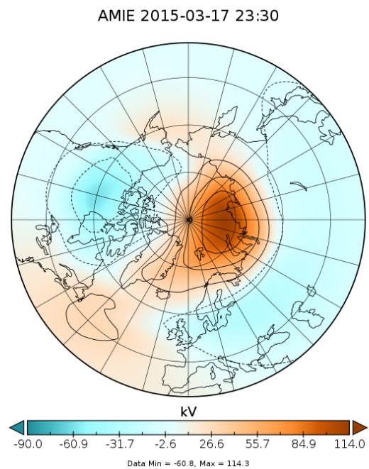
Figure 6. Electric potential maps: Upper-left: Weimer at baseline, Upper-right: AMIE at baseline, Lower-left: Weimer at peak, Lower-right: AMIE at peak
