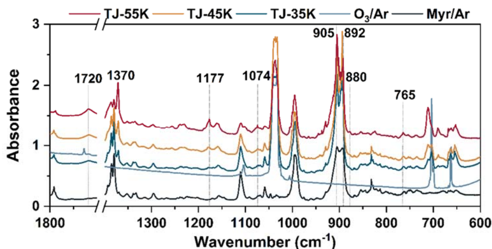
Figure 2 The twin-jet IR spectra of myrcene ozonolysis reaction in a low temperature and Ar matrix after annealing to 35 K, 45 K and 55 K. The blank spectra of myrcene/Ar and O 3 /Ar were also given. T-J means the spectra obtained by twin-jet method.
