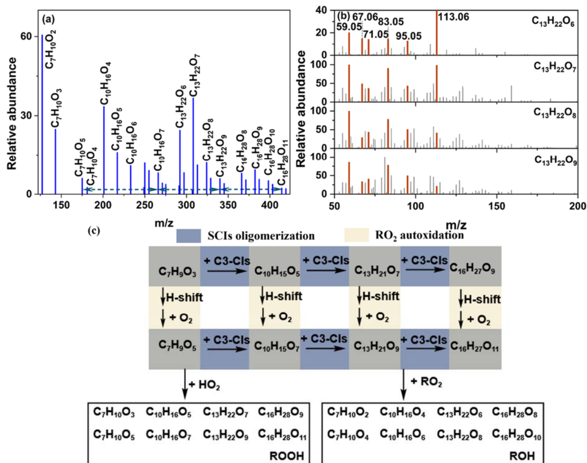
Figure 5 The relative abundance and the proposed pathways of oligomer sequences derived from the synergistic SCIs oligomerization and RO 2 autoxidation. (a) Mass spectrometric distribution of oligomeric sequences under dry conditions. (b) The MS/MS spectra of C 13 H 22 O 6-9 and the major fragment ions were highlighted in orange in the mass spectra. (c) The proposed mechanism of this oligomer sequences. The blue area denoted the SCIs oligomerization pathway. The yellow area represented the RO 2 autoxidation pathway. The black solid box indicated the particulate composition detected by mass spectrometry (MS).
