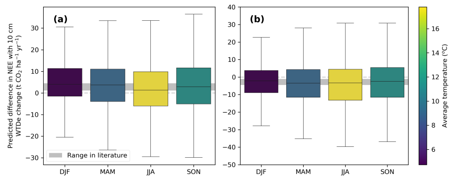
Figure F4. Responses of lowering of WTDe by 10 cm of all sites combined, binned per season. Plot (a) shows the results for 10 cm drier, (b) for 10 cm wetter. Note the different y-axes.
