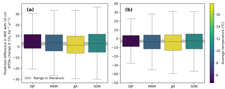
Figure F4. Responses of lowering of WTDe by 10 cm of all sites combined, binned per season. Plot (a) shows the results for 10 cm drier, (b) for 10 cm wetter. Note the different y-axes.
