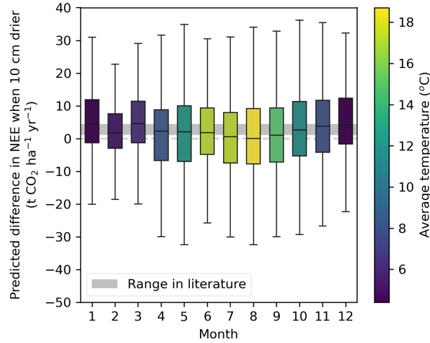
Figure 10. Monthly binned differences in NEE predictions when WTDe increased by 10 cm. The color represents the average temperature in our data for that specific month. The ‘range in literature’ is based on the lowest and highest estimates of the groundwater-CO 2 slopes in the literature: 2.1 t CO 2 ha -1 yr -1 per 10 cm as found by Kruijt et al. (2023) and 4.5 t CO 2 ha -1 yr -1 per 10 cm as found by Fritz et al. (2017). See Fig. 11 and Appendix G for other estimates).
