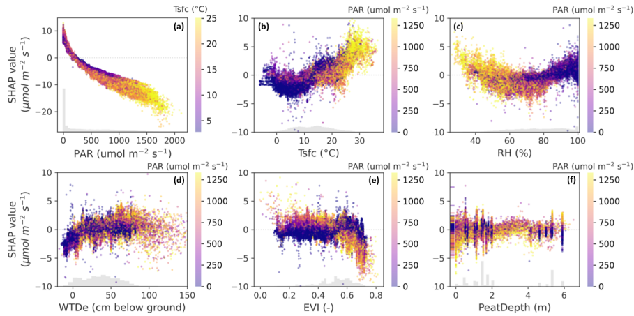
Figure 7. SHAP values of (a) PAR, (b) Tsfc, (c) RH, (d) WTDe, (e) EVI and (f) PeatDepth (for abbreviations, see text or Fig. 6). The plots are colored by the values of another feature (Tsfc in (a), PAR in (b-f)), which in some cases correlates with the depicted one, due to diurnal or seasonal covariance. Nonetheless, the SHAP values represent the effect of only the selected feature on the x-axis. The color gives insight on the conditions in which this effect is happening. The vertical lines in plot ((f) originate from the towers, as a static peat depth map was used. The amount of scatter indicates the robustness of the found relationships.
