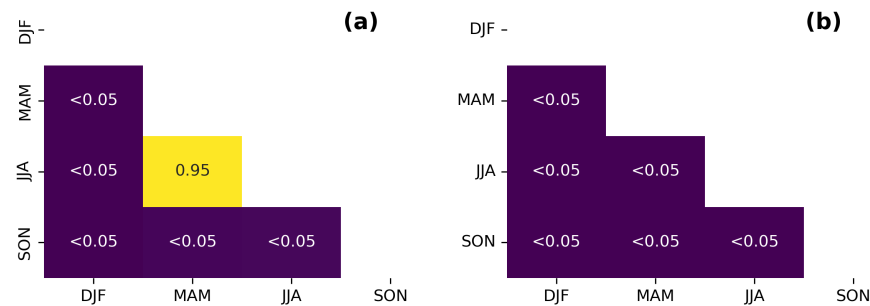
Figure F5. Results of p-values for season-to-season comparison of responses to 10 cm change in WTDe, using Welch's t-test. Plot (a) shows the results for 10 cm drier, (b) for 10 cm wetter.
