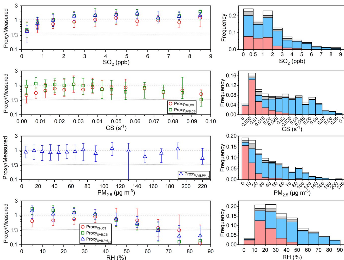
Figure 6. Left: The ratios of sulfuric acid concentrations estimated by proxies in this study to the measured one (Proxy/Measured) vs. concentration of OH radical ( [\text{OH}] ), UVB, \text{SO}_2 , CS, \text{PM}_{2.5} and RH during daytime (10:00-14:00) of 2019. Different colored markers represent different proxies. The up line, middle marker and bottom line stand for upper quartile, median and lower quartile values respectively. Right: Frequency distributions of corresponding parameters classified by “NPF”, “Non-NPF”, “Undefined”, and “No Data” periods.
