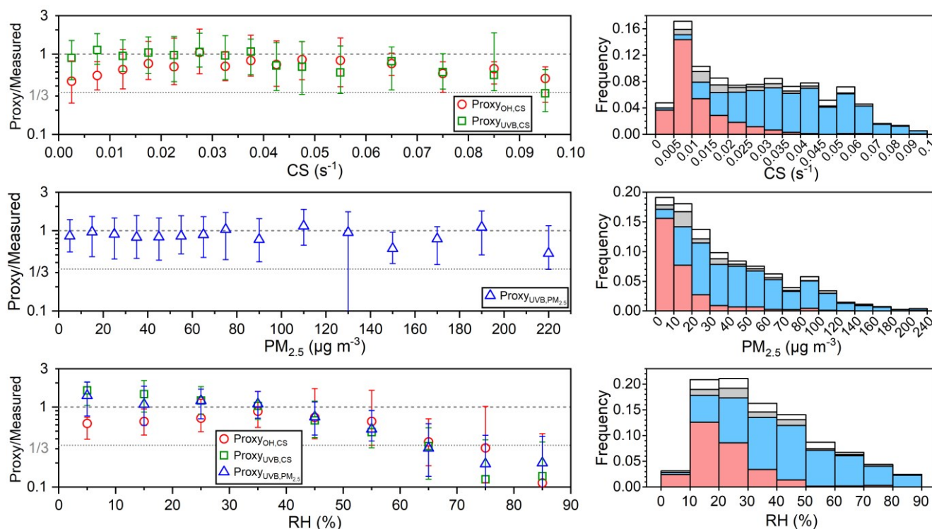
Figure 6. Left: The ratios of sulfuric acid concentrations estimated by proxies in this study to the measured one (Proxy/Measured) vs. concentration of OH radical ( [\text{OH}] ), UVB, \text{SO}_2 , CS, \text{PM}_{2.5} and RH during daytime (10:00-14:00) of 2019. Different colored markers represent different proxies. The up line, middle marker and bottom line stand for upper quartile, median and lower quartile values respectively. Right: Frequency distributions of corresponding parameters classified by “NPF”, “Non-NPF”, “Undefined”, and “No Data” periods.
