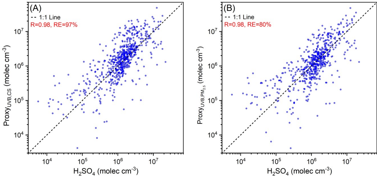
Figure 7. (A) UVB-CS based proxy ( \text{Proxy}_{\text{UVB,CS}} ) and (B) UVB-PM 2.5 based proxy ( \text{Proxy}_{\text{UVB,PM}_{2.5}} ) vs. measured sulfuric acid of Hyytiälä, Finland during daytime (10:00–14:00) from 8 th March to 13 th Aug. 2018. The pre-factor of \text{Proxy}_{\text{UVB,CS}} ( k_{\text{UVB,CS}} ) is 7.5 \times 10^{-6} (\text{T}/300)^{-0.7} \text{W}^{-1} \text{m}^2 \text{s}^{-1} , which is the same as Beijing. The pre-factor of \text{Proxy}_{\text{UVB,PM}_{2.5}} ( k_{\text{UVB,PM}_{2.5}} ) is 4.7 \times 10^{-3} \mu\text{g}^{2/3} \text{W}^{-1} . In both two plots, the black dashed lines are 1:1 lines. Correlation coefficients ( R ) and the relative errors ( \text{RE} ) are shown in the legend.
