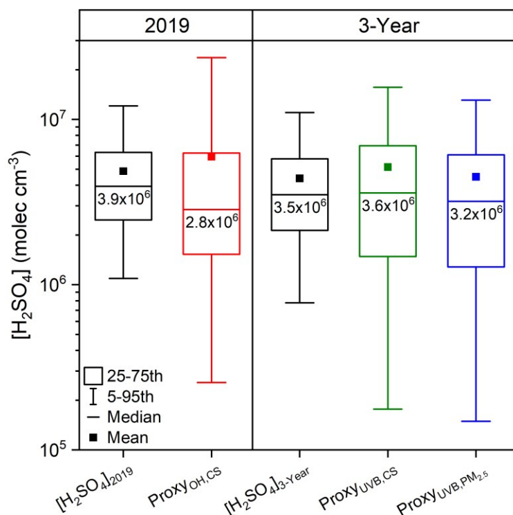
388 Figure 4. Sulfuric acid concentrations from measurement and estimated by proxies in this study during daytime (10:00-14:00). 389
