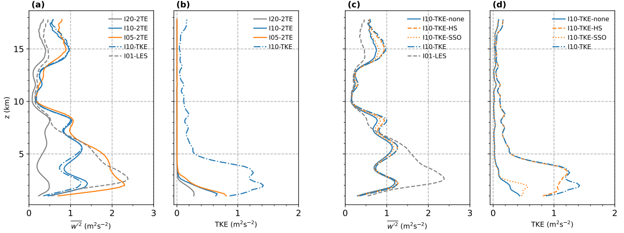
Figure 10. Profiles of resolved vertical velocity variance ( \overline{w'^2} ) and parameterized TKE, averaged over the analysis subdomain shown in Fig. 1, at 18:00 UTC for (a, b) different horizontal resolutions using the 2TE scheme and I10-TKE and (c, d) different TKE-scheme configurations, together with the LES.
