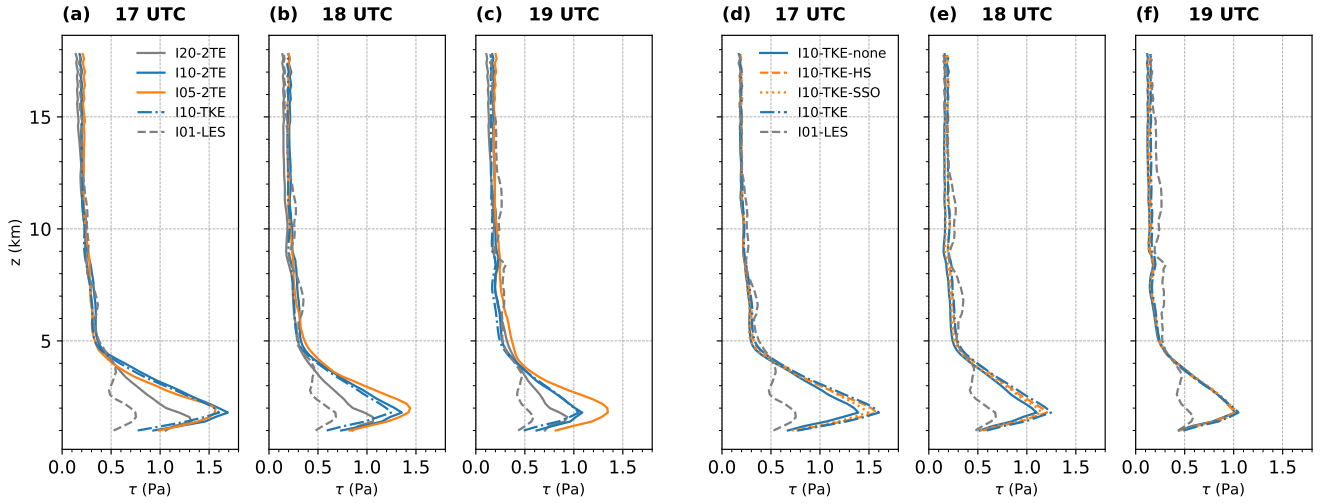
Figure 11. Profiles of area-averaged momentum flux, \tau , for (a–c) different horizontal resolutions using the 2TE scheme and I10-TKE, and (d–f) different TKE-scheme configurations at three consecutive times, together with the LES. Fluxes are calculated within the analysis subdomain shown in Fig. 1 after interpolation to regular vertical levels with 200 m spacing.
