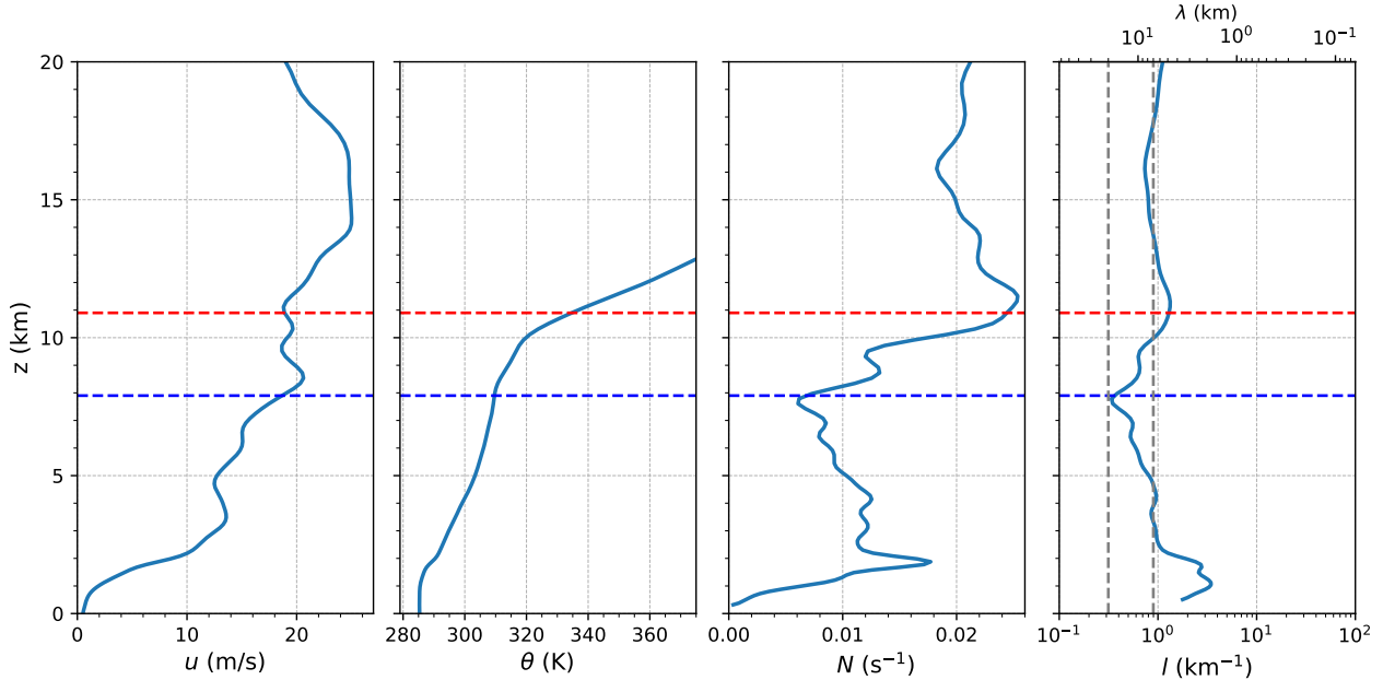
Figure 7. Upstream profiles of wind speed parallel to the southern flight leg ( u ), potential temperature ( \theta ), Brunt–Väisälä frequency ( N ), and Scorer parameter ( l ) from the I10-2TE simulation. Profiles are taken at 10 km along the red transect line shown in Fig. 1 at 18:00 UTC. Wind speed and potential temperature are smoothed vertically using a Gaussian filter with a standard deviation of 1.5 vertical grid points. The grey vertical dashed lines indicate a Scorer parameter values corresponding to wavelengths of 7 and 20 km, respectively.
