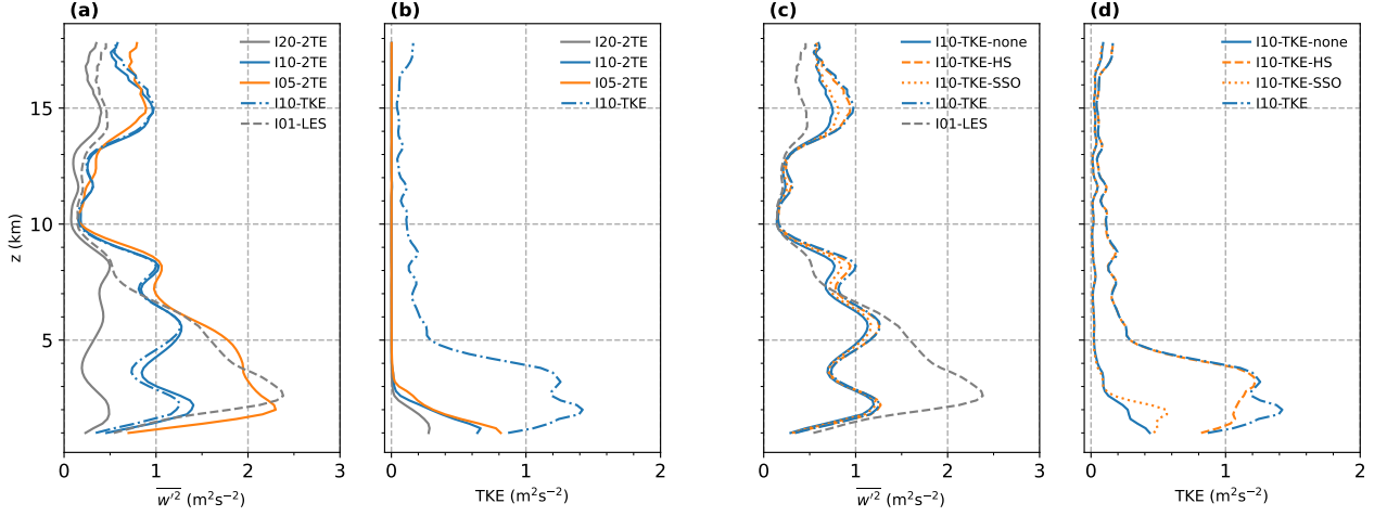
Figure 9. Profiles of resolved vertical velocity variance ( \overline{w'^2} ) and parameterized TKE, averaged over the analysis subdomain shown in Fig. 1, at 18:00 UTC for (a, b) different horizontal resolutions using the 2TE scheme and I10-TKE and (c, d) different TKE-scheme configurations, together with the LES.
