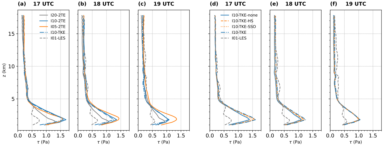
Figure 10. Profiles of area-averaged momentum flux, \tau , for (a–c) different horizontal resolutions using the 2TE scheme and I10-TKE, and (d–f) different TKE-scheme configurations at three consecutive times, together with the LES. Fluxes are calculated within the analysis subdomain shown in Fig. 1 after interpolation to regular vertical levels with 200 m spacing.
