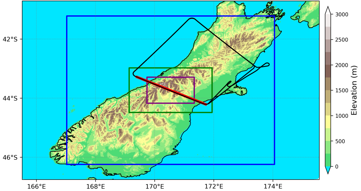
Figure 1. Orography (color shading) and simulation domains for the nested ICON setup: 1 km (full region), 500 m (blue box), and 130 m for the southern flight segment (green box). The red line marks the cross-section along the flight path used for the main analysis, and the purple box indicates the averaging region for calculating bulk properties of the GW field (Sect. 3.4). The black solid line shows the full flight path of research flight FF09 of the Falcon aircraft on 12 July 2014 (17:15–20:15 UTC) during the DEEPWAVE campaign.
