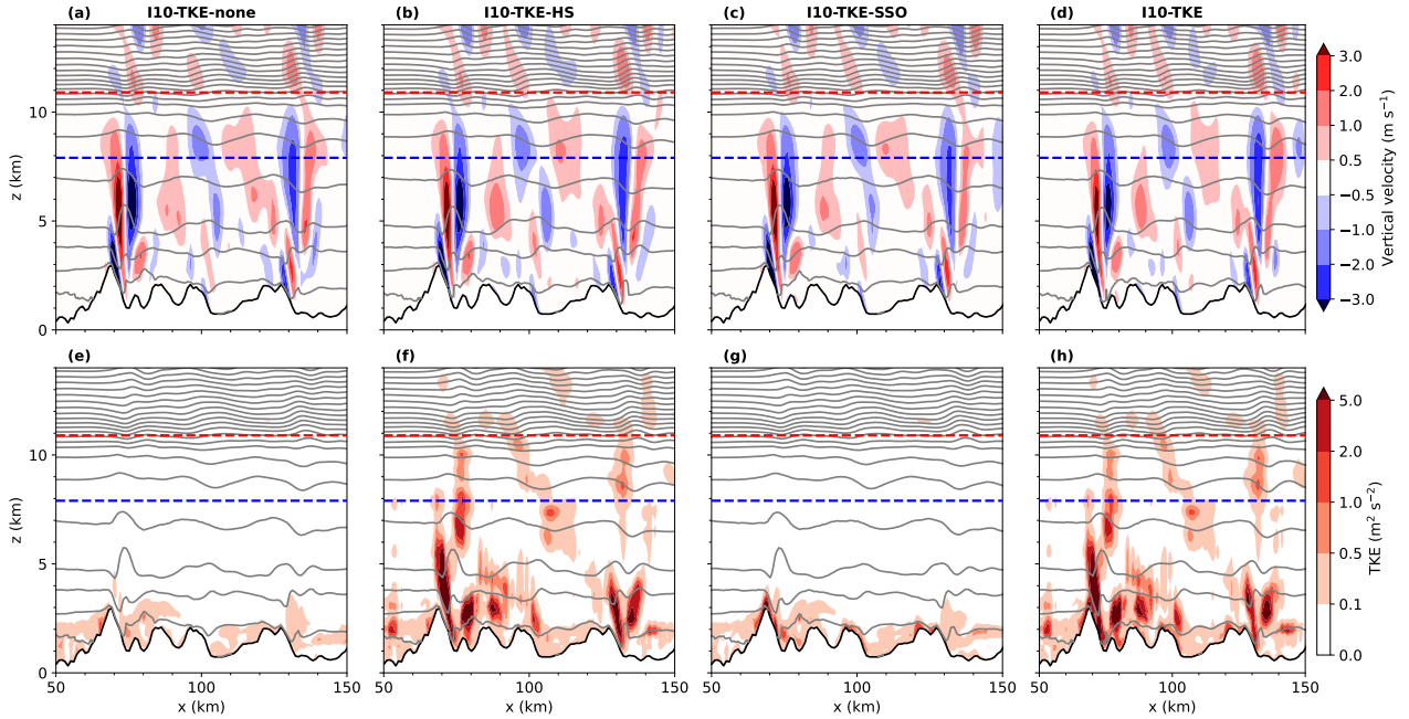
Figure 8. Comparison of vertical velocity and TKE along the southern flight-path transect at 18:00 UTC for ICON simulations using the TKE scheme: (a, e) both horizontal shear (HS) and subgrid-scale orography (SSO) deactivated, (b, f) HS activated, (c, g) SSO activated, and (d, h) both HS and SSO activated (standard operational configuration).
