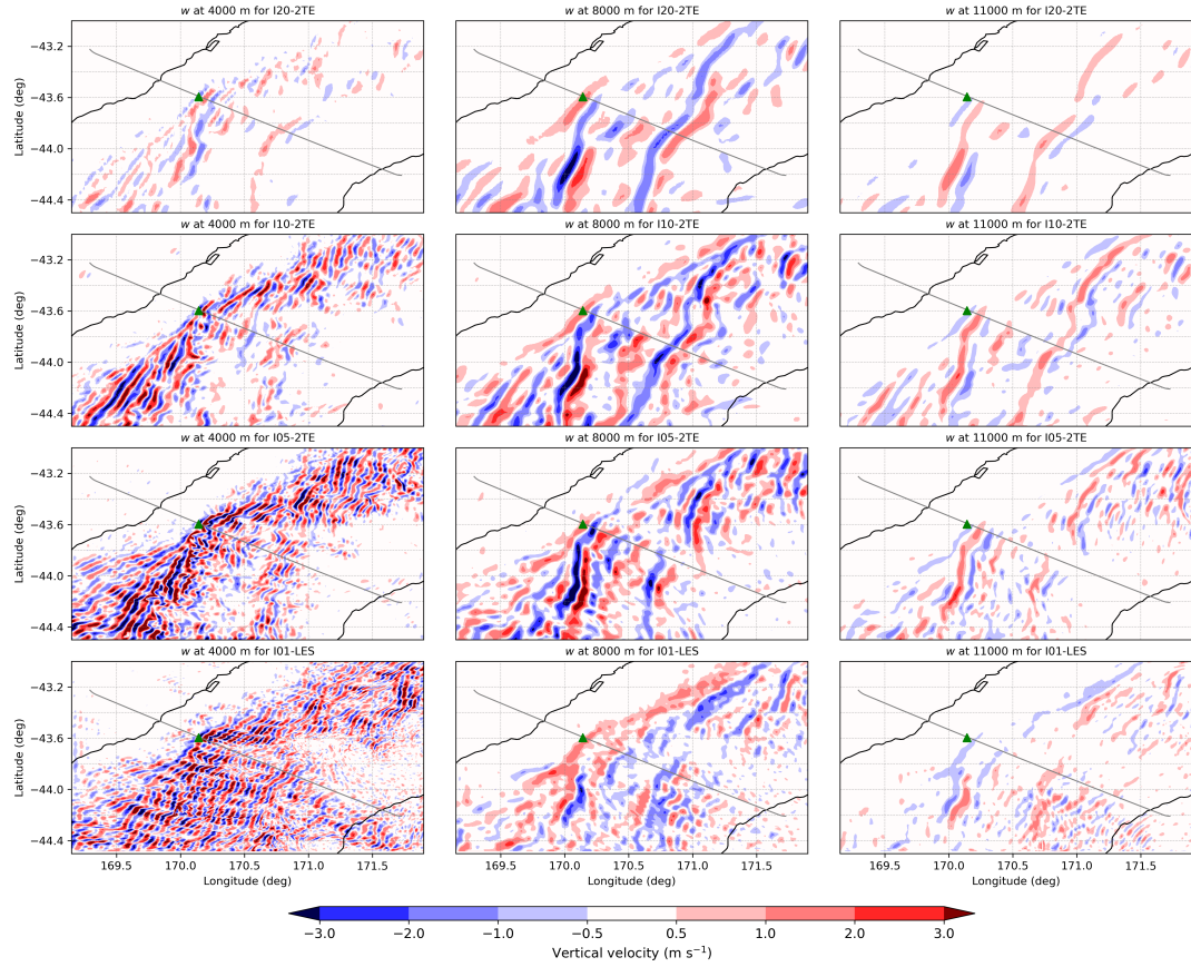
Figure B1. Horizontal cross-sections of vertical velocity at 8000 m and 11 000 m, corresponding to the lower and upper flight legs, for ICON simulations using the 2TE turbulence scheme at different horizontal resolutions, together with the LES.
