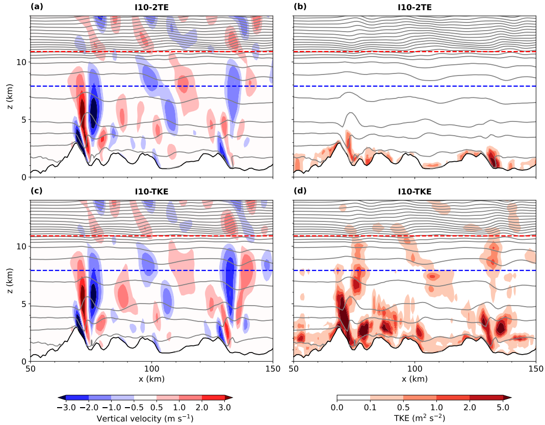
Figure 7. Comparison of vertical velocity and TKE along the southern flight-path transect at 18:00 UTC for ICON simulations at 1 km resolution using (a, b) the 2TE scheme and (c, d) the TKE scheme.
