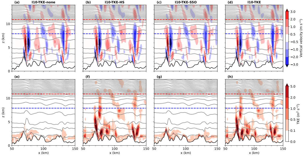
Figure 9. Comparison of vertical velocity and TKE along the southern flight-path transect at 18:00 UTC for ICON simulations using the TKE scheme: (a, e) both horizontal shear (HS) and subgrid-scale orography (SSO) deactivated, (b, f) HS activated, (c, g) SSO activated, and (d, h) both HS and SSO activated (standard operational configuration).
