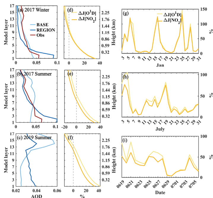
Figure 2. Vertical profiles of average (a–c) AOD, (d–f) relative changes of J[NO_2] , and J[O^1D] in model layers at observation stations. The red, light, and dark blue lines represent observed, BASE simulated, and REGION simulated AOD, respectively. (g–i) Time series of daily average relative changes of surface J[NO_2] , and J[O^1D] at observation stations. From top to bottom are for winter 2017 (a, d, g), summer 2017 (b, e, h), and summer 2019 (c, f, i), respectively. The averages are calculated using data during the daytime when photolysis occurs.
