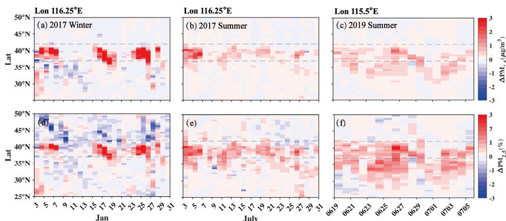
Figure 9. Simulated responses of daily average (daytime) PM_{2.5} to observational constraints on aerosol vertical distribution along the longitude profiles of observation stations. Top panel: mass concentration ( \mu g m^{-3} ); Bottom panel: proportion (%). From left to right are for winter 2017 (a, d), summer 2017 (b, e), and summer 2019 (c, f), respectively. The dotted lines indicate the latitude range of the modified region, and the longitudes of the stations are marked at the top.
