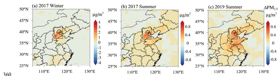
Figure 8. Simulated responses of PM_{2.5} concentration to observational constraints on aerosol vertical distribution over North China. From left to right are for winter 2017 (a), summer 2017 (b), and summer 2019 (c), respectively. The black rectangle shows the region where vertical distribution modification was performed.
