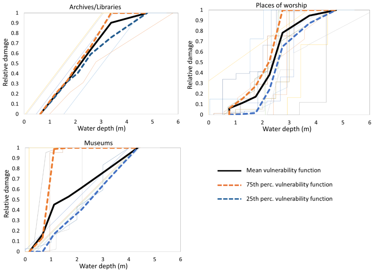
Fig. 6 Artworks vulnerability functions for libraries/archives (top left), places of worship (top right) and museums (bottom left). The bold black, orange and blue curves are the average, 75th and 25th percentile vulnerability functions.
