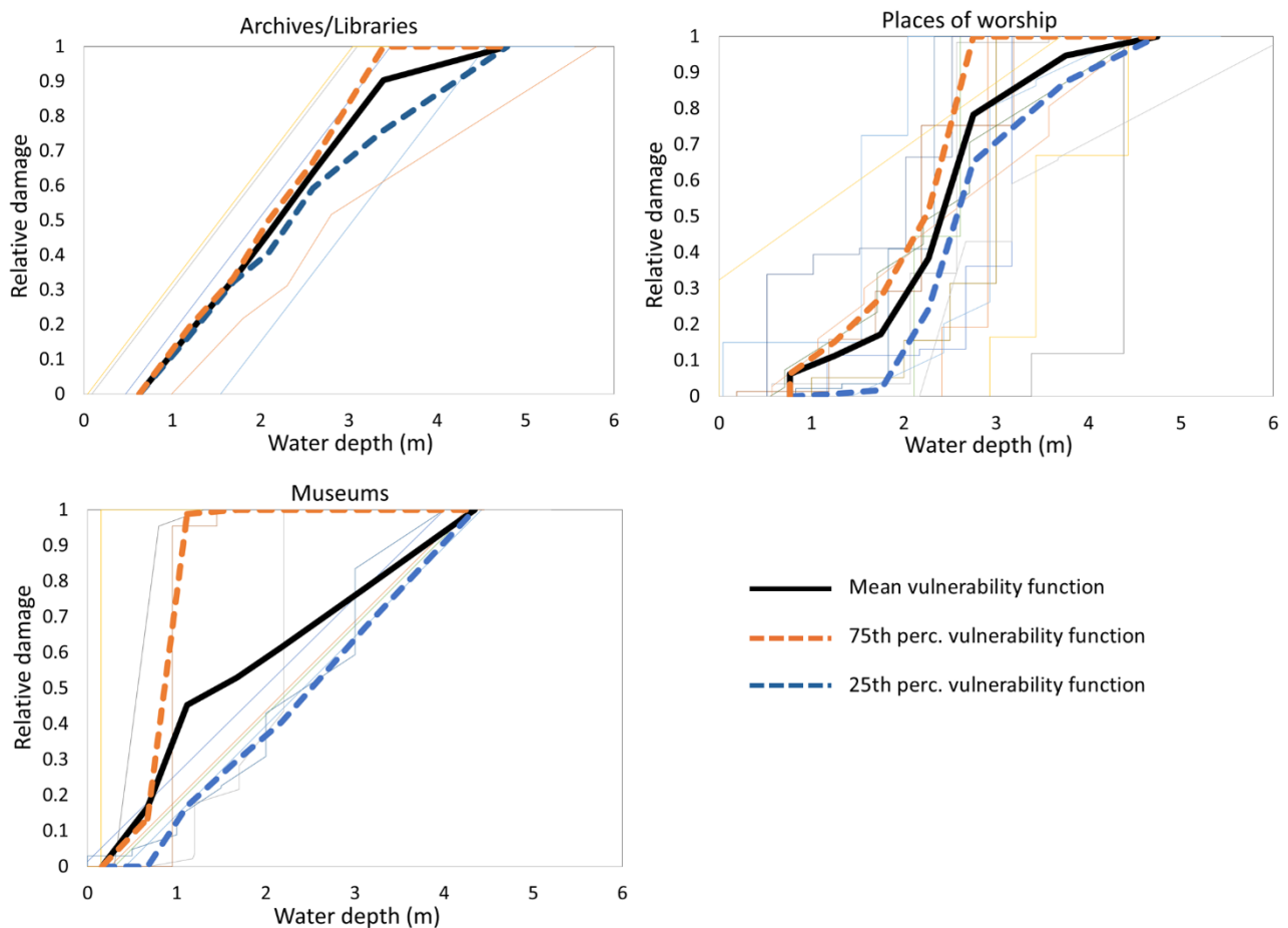
490 Fig. 6 Artworks vulnerability functions for libraries/archives (top left), places of worship (top right) and museums (bottom left). The bold black, orange and blue curves are the average, 75th and 25th percentile vulnerability functions.
