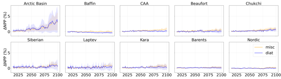
Figure A6: Projected NPP relative to 1995-2014 during the period 2015-2100 of SSP5-8.5 in each basin of the Arctic Ocean. Diatoms are represented in blue and miscellaneous phytoplankton in orange. Shading represents the multi-model standard deviation.
