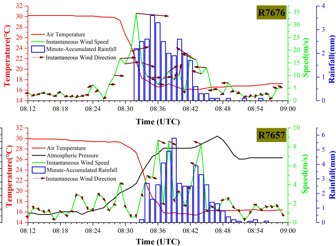
Figure 5: Time Series of Meteorological Observation Elements at Huawucun Station (R7676) and Baili Gallery Station (R7657)
