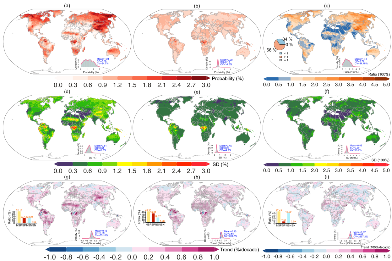
Figure 7. Spatial distributions of the mean observed probability (a), mean random probability
