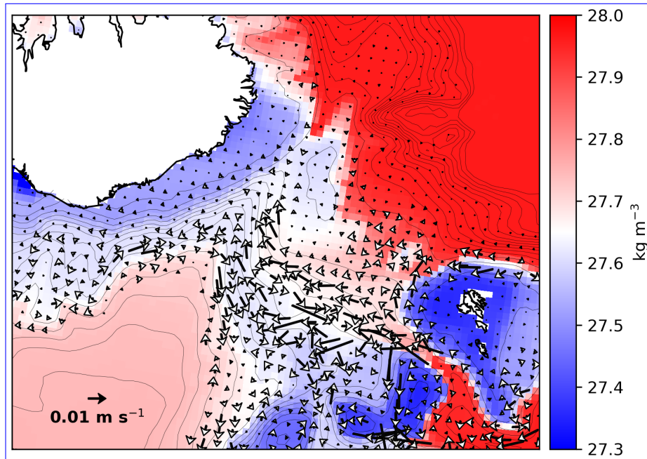
Figure 4. Comparison of bottom density between the DPLUME-Full parameterization on bottom velocities, compared with previously-existing-BBL-parameterizations-the NOBBL reference. Comparison of NEMO bottom velocities EMO. a) Colourscale: NOBBL Bottom Density. Vectors: difference of bottom velocity between DPLUME-FULL and NOBBL experiments, only represented for depth above 2000m b) DPLUME-FULL minus NOBBL c) DPLUME-FULL minus DIFF d) DPLUME-FULL minus ADV1 e) DPLUME-FULL minus ADV2
