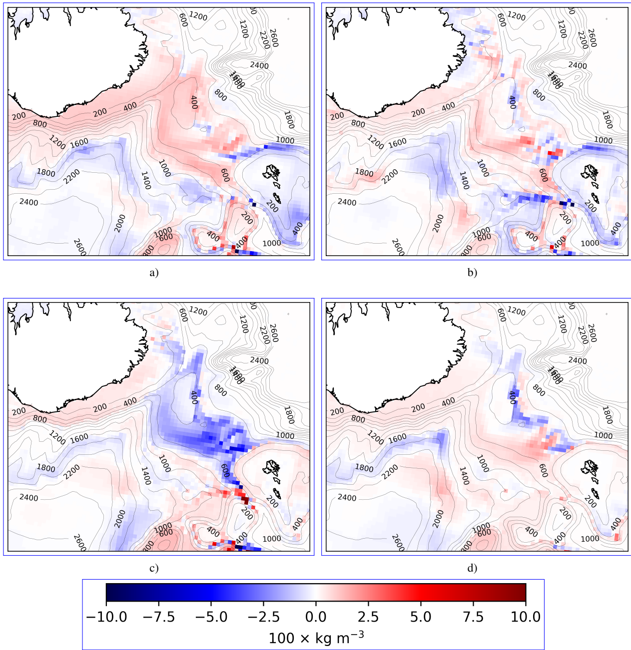
Figure 6. Comparison of bottom density between the DPLUME-Full parameterization with previously existing BBL parameterizations of NEMO. a) DPLUME-Full minus NOBBL b) DPLUME-Full minus BD c) DPLUME-Full minus CG_ADV1 d) DPLUME-Full minus CG_ADV2
