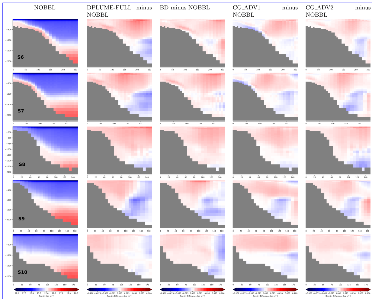
Figure A2. Continuation of Figure A1
