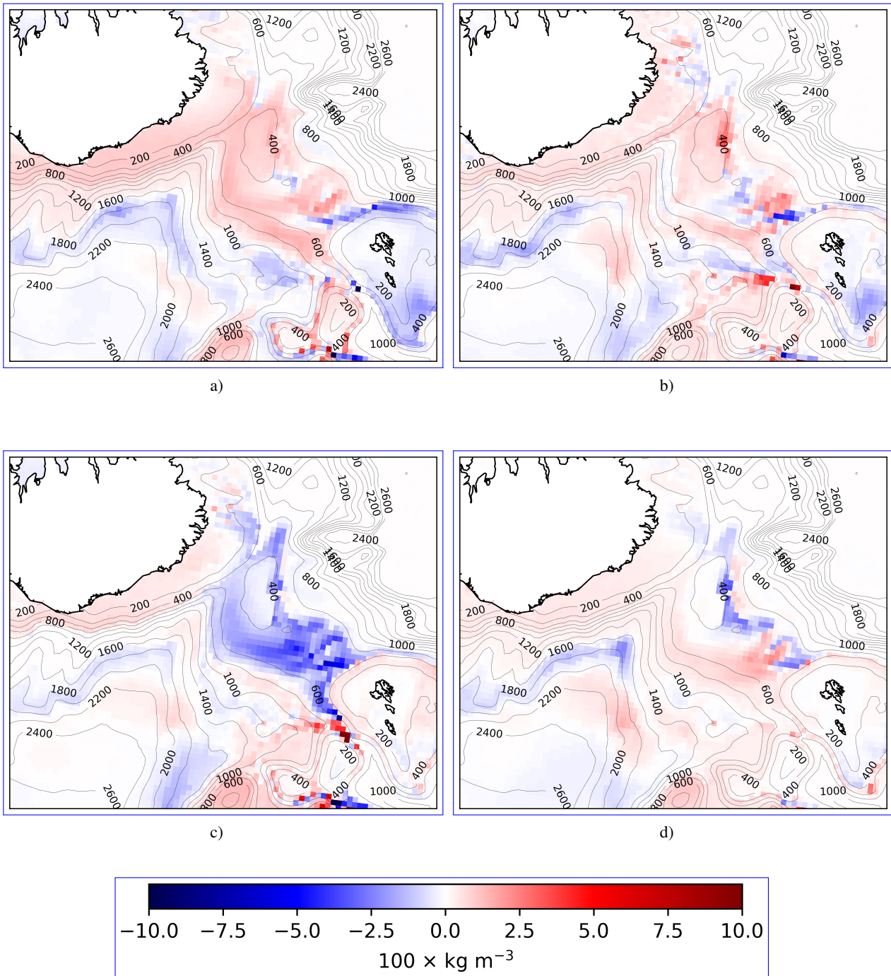
Figure 5. Comparison of bottom density between several BBL parameterizations. a) DPLUME-Full minus NOBBL b) BD minus NOBBL c) CG_ADV1 minus NOBBL d) CG_ADV2 minus NOBBL
