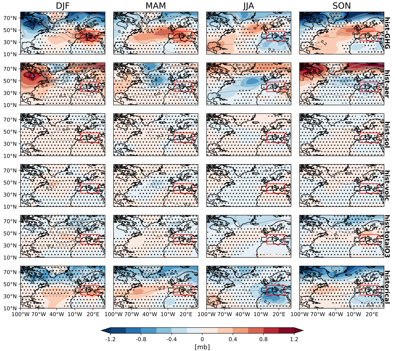
Figure 1. Multi-model means of the seasonal (column-wise) PSL responses (1990-2014 vs. 1851-1920) in the single-forcing and all-forcings experiments (row-wise). The red rectangle marks the Mediterranean region as defined in the main text. Regions without stippling indicate where at least 80% of the models agree on the sign of the response. Gray contours quantify the multi-model standard deviation and indicate the intermodel spread. Similar figures but for different averaging periods are shown in Supplemental Figure S1.
