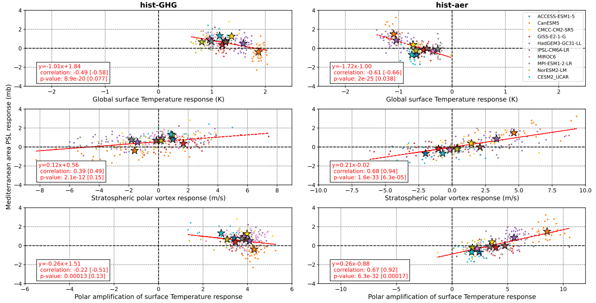
DJF Mediterranean area PSL response vs. Global T2m/10mb polar vortex/Polar amplification of T2m responses; 1990-2014 vs 1850-1920
