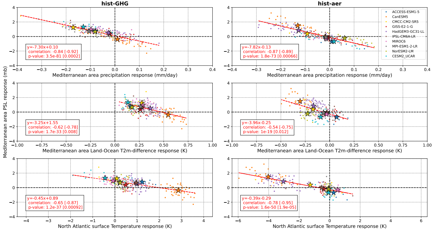
DJF Mediterranean area PSL response vs. precipitation/land-ocean T2m-difference/NA T2m responses; 1990-2014 vs 1850-1920
