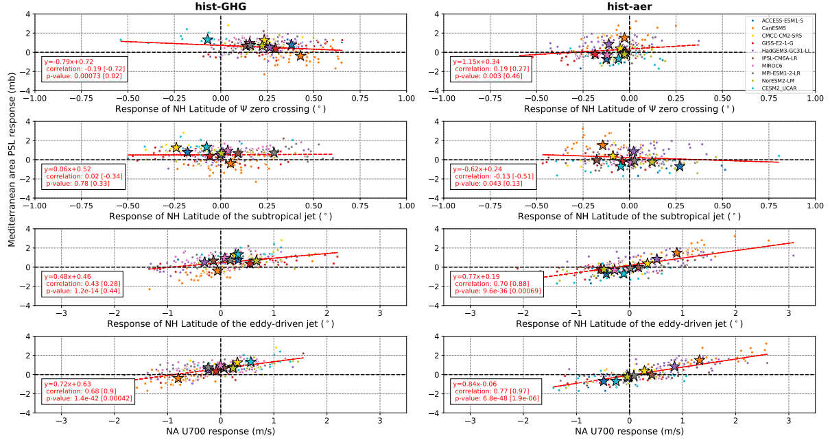
DJF Mediterranean area PSL response vs. responses of Northern Hemisphere Latitude of tropical belt edge and U700; 1990-2014 vs 1851-1920
