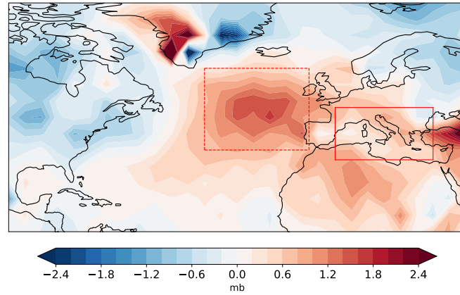
DJF PSL observations response, 1990-2014 vs. 1851-1920
