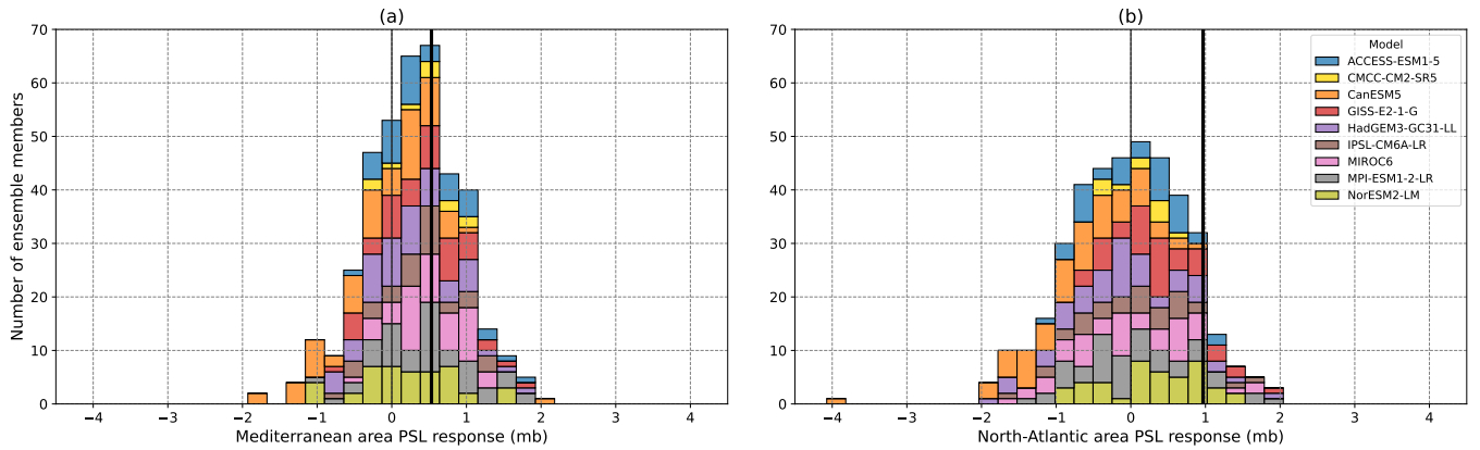
DJF historical PSL response distributions; Mediterranean and NA regions; 1990-2014 vs 1850-1920
