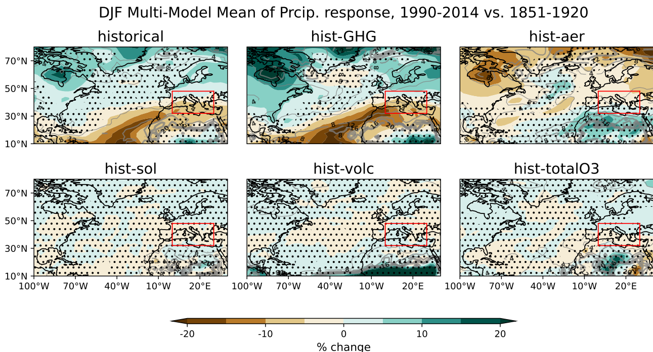
Figure 4. Multi-model means of the seasonal (column-wise) DJF precipitation responses (1990-2014 vs. 1851-1920) in the single-forcing experiments (row-wise). The red rectangle marks the Mediterranean region as defined in the main text. Regions without stippling indicates where at least 80% of the models agree on the sign of the response. Gray contours quantify the multi-model standard deviation and indicate the intermodel spread. Similar figures but for a different averaging period are A similar figure including the other seasons is shown in Supplemental Figure S2S5 .
