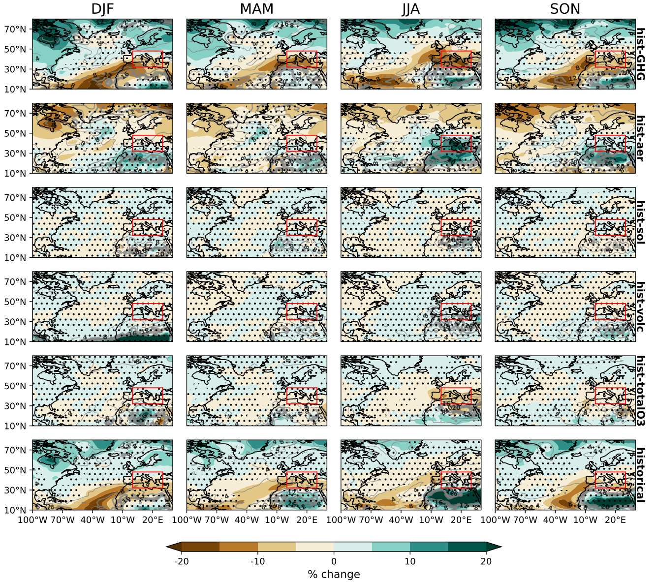
Figure 4. Multi-model means of the seasonal (column-wise) precipitation responses (1990-2014 vs. 1851-1920) in the single-forcing experiments (row-wise). The red rectangle marks the Mediterranean region as defined in the main text. Regions without stippling indicates where at least 80% of the models agree on the sign of the response. Gray contours quantify the multi-model standard deviation and indicate the intermodel spread. Similar figures but for a different averaging period are shown in Supplemental Figure S2.
