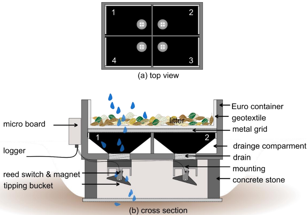
170 Figure 2: Design of FluxIT sampler with four equal drainage compartments (top view), each equipped with single tipping bucket units for measurement (cross section). Photographs (c, d) show samplers installed at two locations in the field, at a moment of configuration II for measurements of integrated throughfall with litter in the samplers
