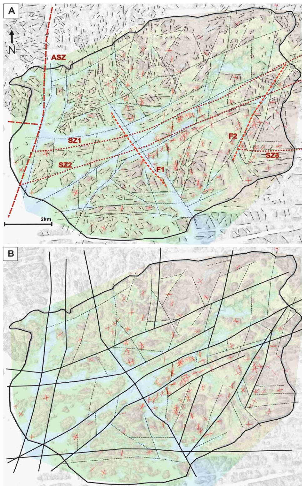
Figure 9. Compilation of brittle structures and their relationship with shear zones and faults. Ground surface LiDAR and Bedrock-DEM on the background (transparent colour map equivalent with the Fig. 8). Black dashed lines = elongated bedrock depressions, red lines= fracture measurements. A) Shear zones 1-3 (red-dotted lines) and Faults 1-2 (red-dashed lines) detected from the low-altitude aeromagnetic data and lidar lineaments = black lines, B) The network of shear zones and faults (Black solid lines).
