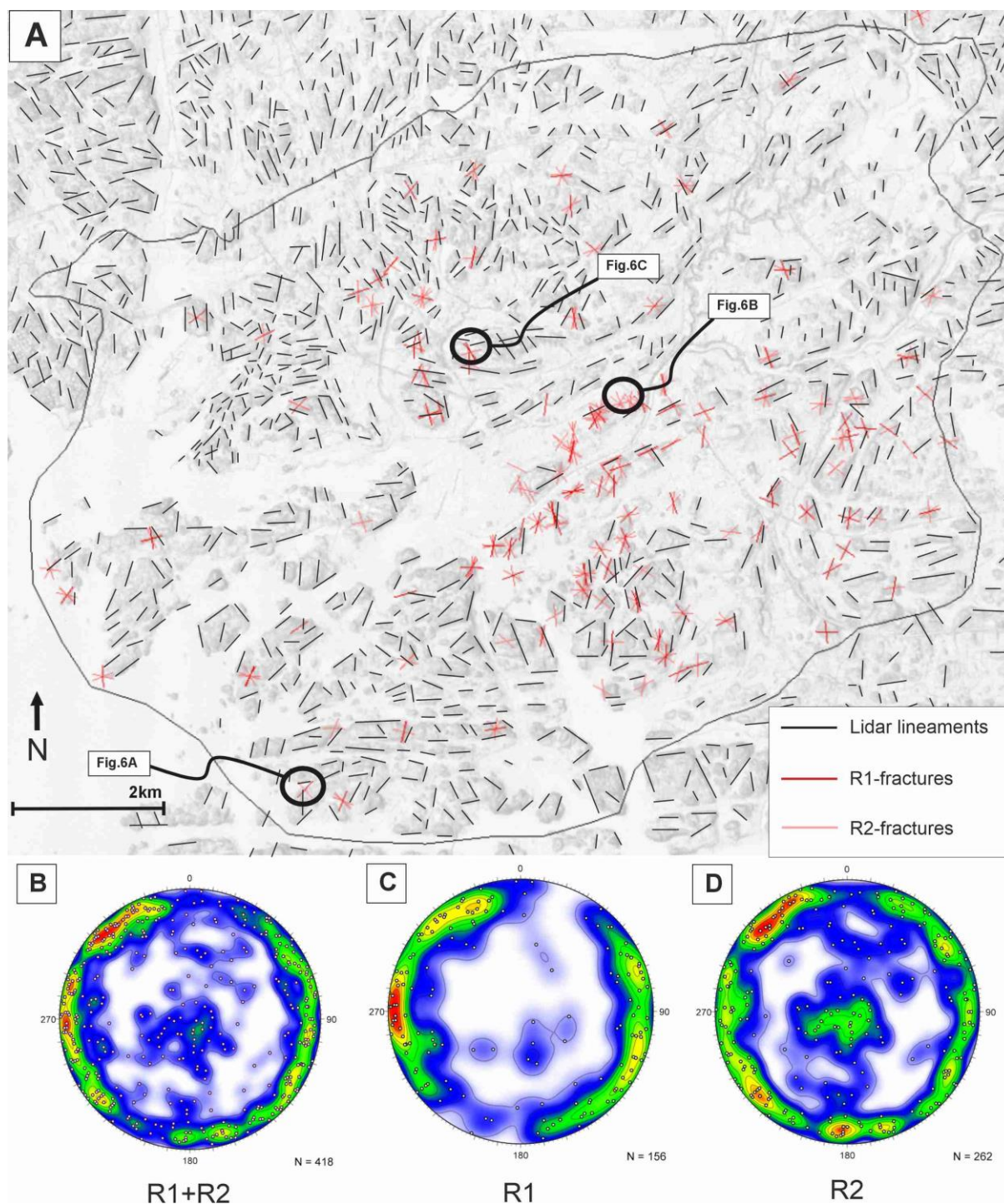
Figure 6. Brittle structures within the study area. A) Lidar lineaments and outcrop fractures. Ground surface elevation LiDAR on the background. Stereoplots represent all of the fractures (B), R1-fractures (C) and R2-fractures (D).
