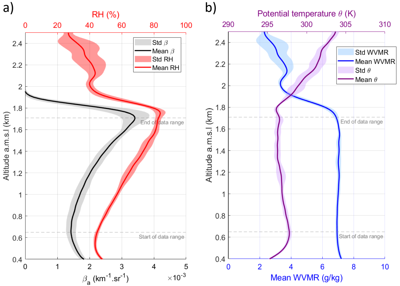
345 Figure 3. Atmospheric parameters for case study 3 as a function of the altitude a.m.s.l.: a) the vertical profile of the backscattering coefficient in black and RH in red, b) the Water Vapour Mixing Ratio (WVMR) in blue, the potential temperature ( \theta ) in purple. The shaded areas represent the standard deviation of the data considered. Grey dotted lines give the altitude range considered. Case study 3 serves as a reference in terms of atmospheric conditions for the study of hygroscopicity. All the case studies present similar atmospheric conditions.
