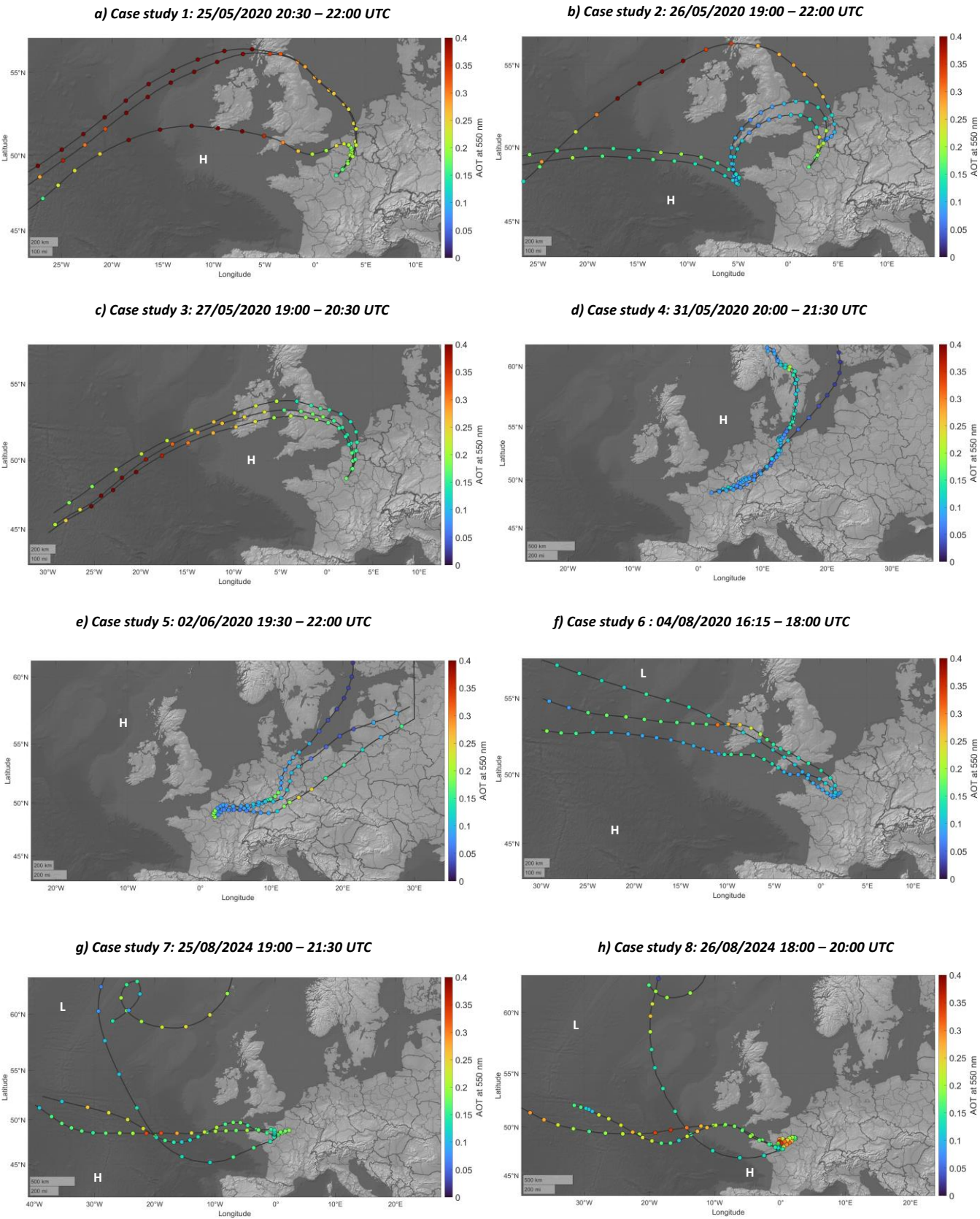
360 Figure 5. Five-days air mass back trajectories for the 8 hygroscopic case studies. The 3 lines represent 3 of the HYSPLIT ensemble mode whose arrival point is set in the time interval of each case study and at the middle of the studied aerosol layer. Each coloured dot corresponds to the Aerosol Optical Thickness (AOT) given by CAMS reanalysis on the date corresponding to the HYSPLIT points. Each point on each trajectory is 3 hours apart. The letters 'H' and 'L' indicate the locations of high and low systems at 850 hPa, respectively.
