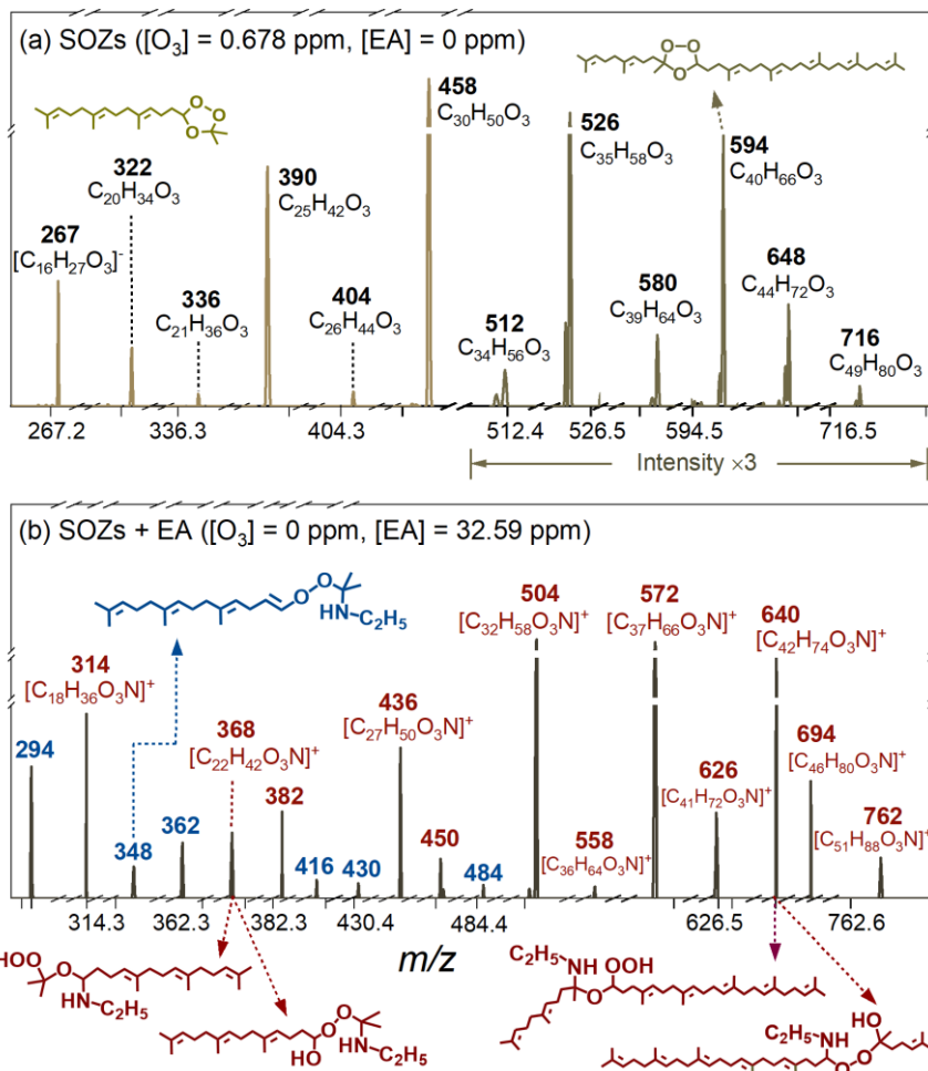
Figure 3: Mass spectra of (a) representative SOZs (the signals within m/z range of 500-800 are amplified) formed during the ozonolysis of Sqe in the first flowtube reactor, and (b) their amination products (adducts of SOZ + EA are in red and dehydration products are in blue) upon exposure to ethylamine (EA) in the secondary flowtube reactor.
