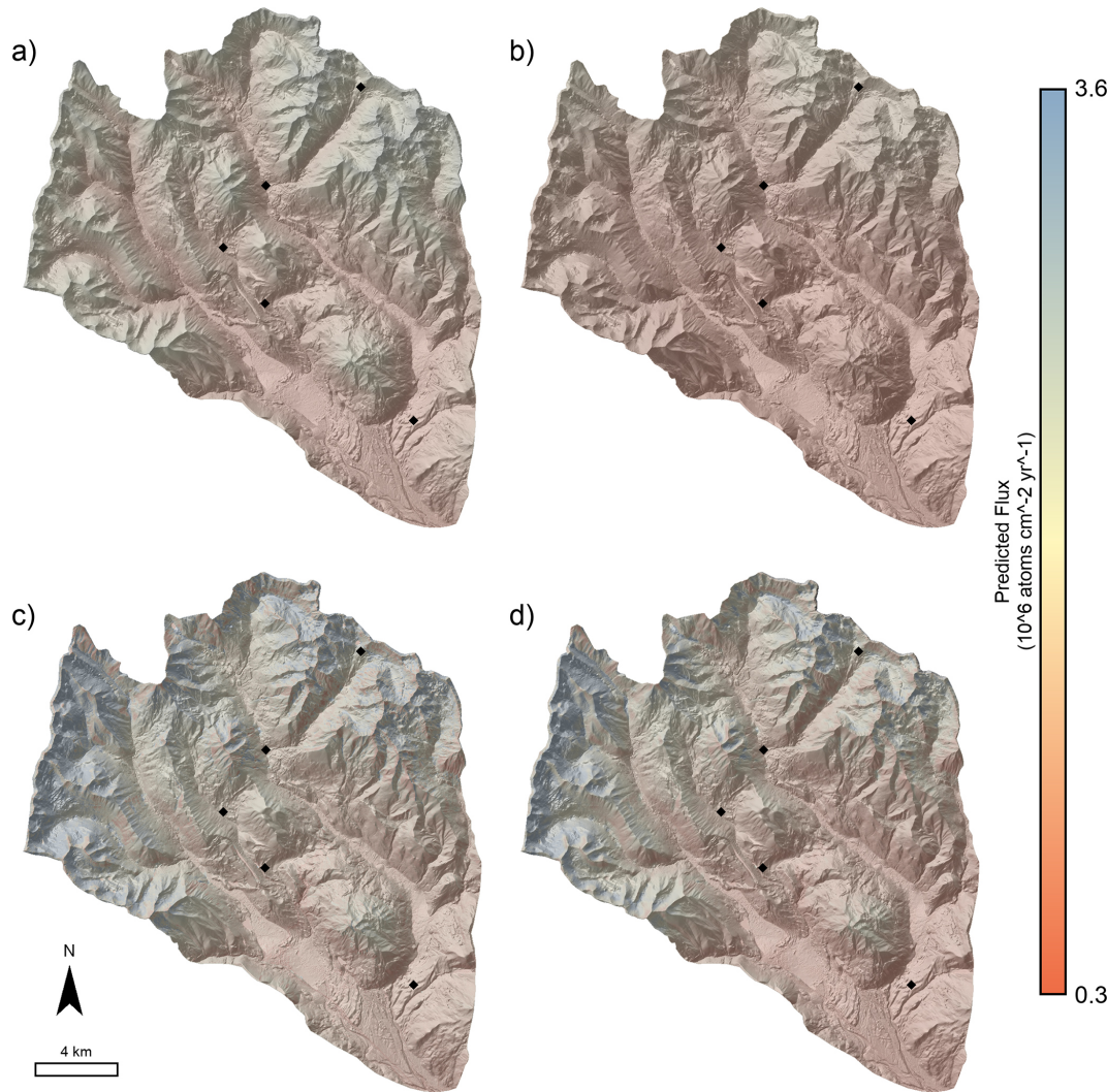
Figure 5. Spatial predictions of ^{10}\text{Be}_{\text{met}} flux based on inheritance-corrected regression models using: (a) elevation with the regular regression; (b) mean annual precipitation with the origin regression; (c) mean snow depth from 2018–2019 with the origin regression; and (d) mean snow water equivalent from 2018–2019 with the origin regression. The equivalent results for erosion- and desorption-corrected fluxes calculated using the profile-average desorption model are shown in Fig. S6.
