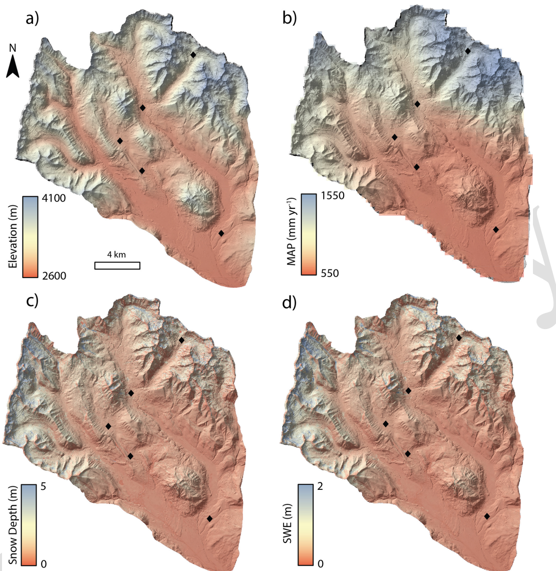
Figure 2. Maps of environmental variables within the East River watershed. (a) LiDAR-derived elevation data (Goulden et al., 2020); (b) downscaled Precipitation-elevation Regressions on Independent Slopes Model (PRISM) mean annual precipitation (MAP) data averaged from 2008–2019 (Mital et al., 2022); (c) mean snow depth, and (d) mean snow water equivalent (SWE), derived from Airborne Snow Observatory data from 2018–2019 (Painter, 2018a, b). The black diamonds show each sample location.
