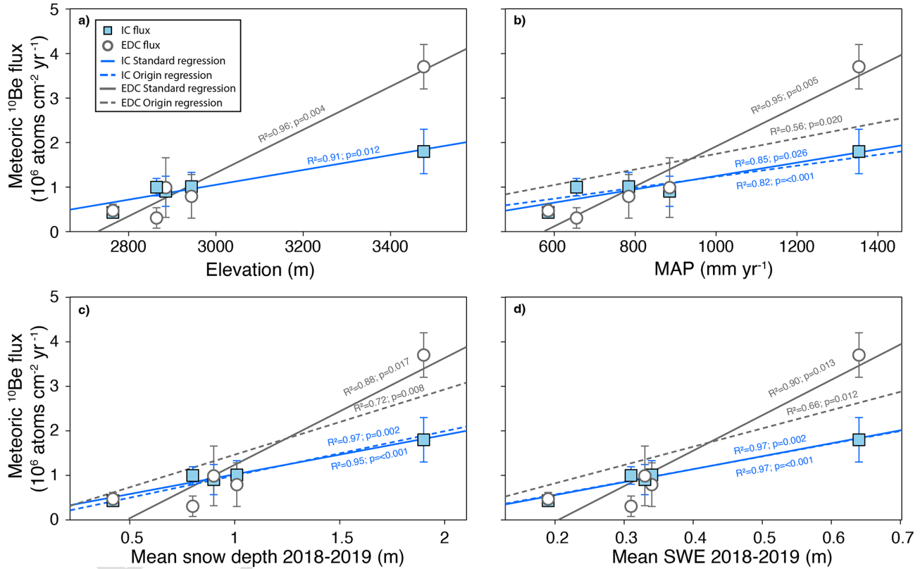
Figure 4. Linear regression models of ^{10}\text{Be}_{\text{met}} flux versus (a) elevation, (b) mean annual precipitation (MAP), (c) mean snow depth (2018–2019), and (d) mean snow water equivalent (SWE) (2018–2019). Blue squares show inheritance-corrected fluxes and open gray circles show erosion- and desorption-corrected fluxes. The erosion- and desorption-corrected fluxes use the profile-average desorption model. For the inheritance-corrected (IC) data, solid blue lines show results from standard regression models and the dashed blue lines show regression through the origin models. For the corrected (EDC) data, solid grey lines show standard regression model results and grey dashed lines show regression through the origin models where the y-intercept is zero. Regression through the origin models are shown only for MAP, mean snow depth, and mean SWE. Regression coefficients, R^2 values, and p values are reported in Table S6. Figure S3 and Table S7 report regression results with Copper Creek excluded from the analysis. Figures S4 and S5 show the results from the uppermost and lowermost sample desorption models.
