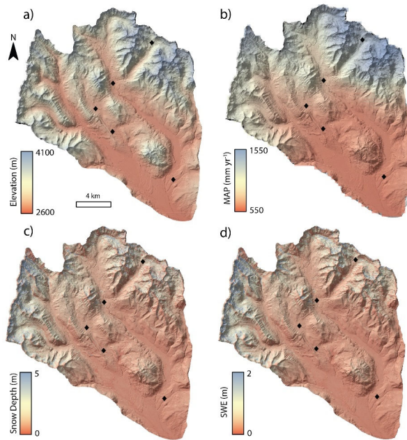
Figure 2: Maps of environmental variables within the East River watershed. (a) LiDAR-derived elevation data; (Goulden et al., 2020); (b) Mean downscaled Precipitation-elevation Regressions on Independent Slopes Model (PRISM) mean annual precipitation (MAP) data averaged from 2008–2019; (Mital et al., 2022); (c) Mean mean snow depth, and (d) Mean mean snow water equivalent (SWE), derived from Airborne Snow Observatory data from 2018–2019; (Painter et al., 2018a, b). The black diamonds show each sample location.
