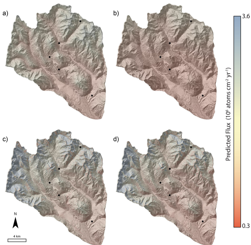
Figure 65. Spatial predictions of ^{10}\text{Be}_{\text{net}} flux based on inheritance-corrected regression models using: (a) elevation with the regular regression; (b) mean annual precipitation with the origin regression; (c) mean snow depth from 2018–2019 with the regular regression; (d) mean snow depth from 2018–2019 with the origin regression.
