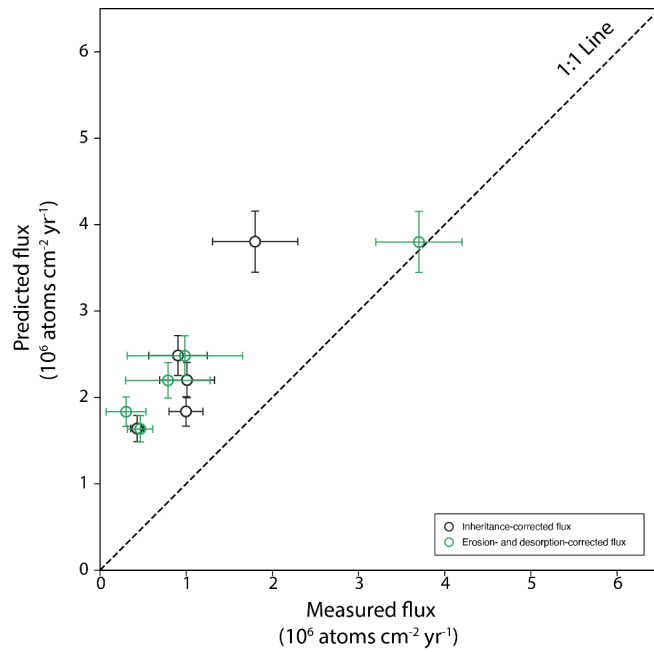
Figure 76. Predicted ^{10}\text{Be}_{\text{met}} flux from the empirical precipitation-based model of Graly et al. (2011), scaled to reflect Holocene-average values (e.g., Clow et al., 2020) versus measured flux values for the five study sites. Measured erosion- and desorption-corrected fluxes use the profile-average desorption model.
