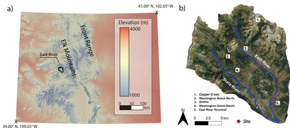
130 Figure 1: a) Digital elevation model (DEM) of Colorado, USA showing the location of East River watershed. b) Image of the East River watershed showing locations (red diamonds) where soil ^{10}\text{Be}_{\text{met}} inventories and fluxes were measured.
