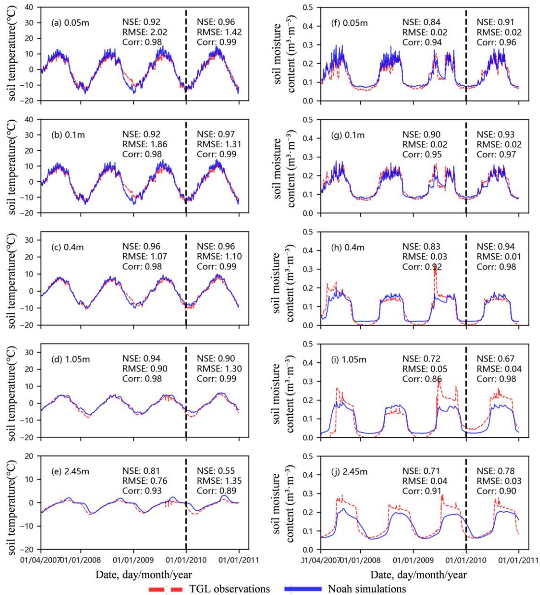
310 Figure 4. Simulated and observed daily soil temperature and liquid soil water content at various depths (daily; 0.05, 0.1, 0.4, 1.05, and 2.45m) for the Tanggula (TGL) site. The vertical black dashed line separates the calibration period (April 1, 2007–December 31, 2009) from the validation period (January 1, 2010–December 31, 2010). Inset text in each panel provides the NSE, RMSE, and correlation coefficient (Corr) for both periods.
