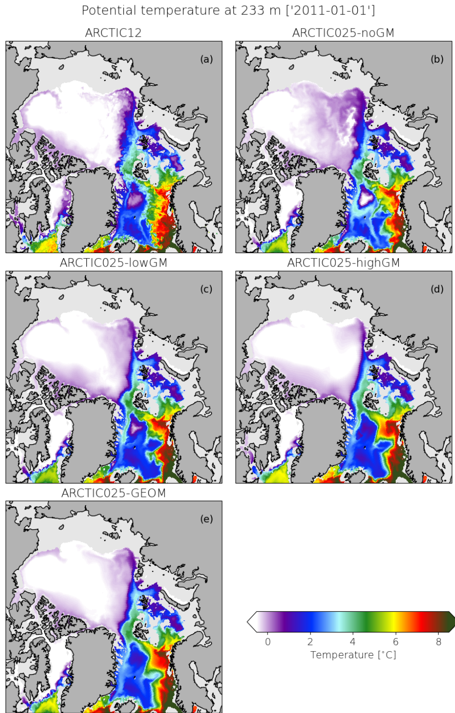
Figure A2. Daily snapshot (1st of January 2011) of potential temperature in the Atlantic Water layer (233 m depth) computed for the different experiments.
