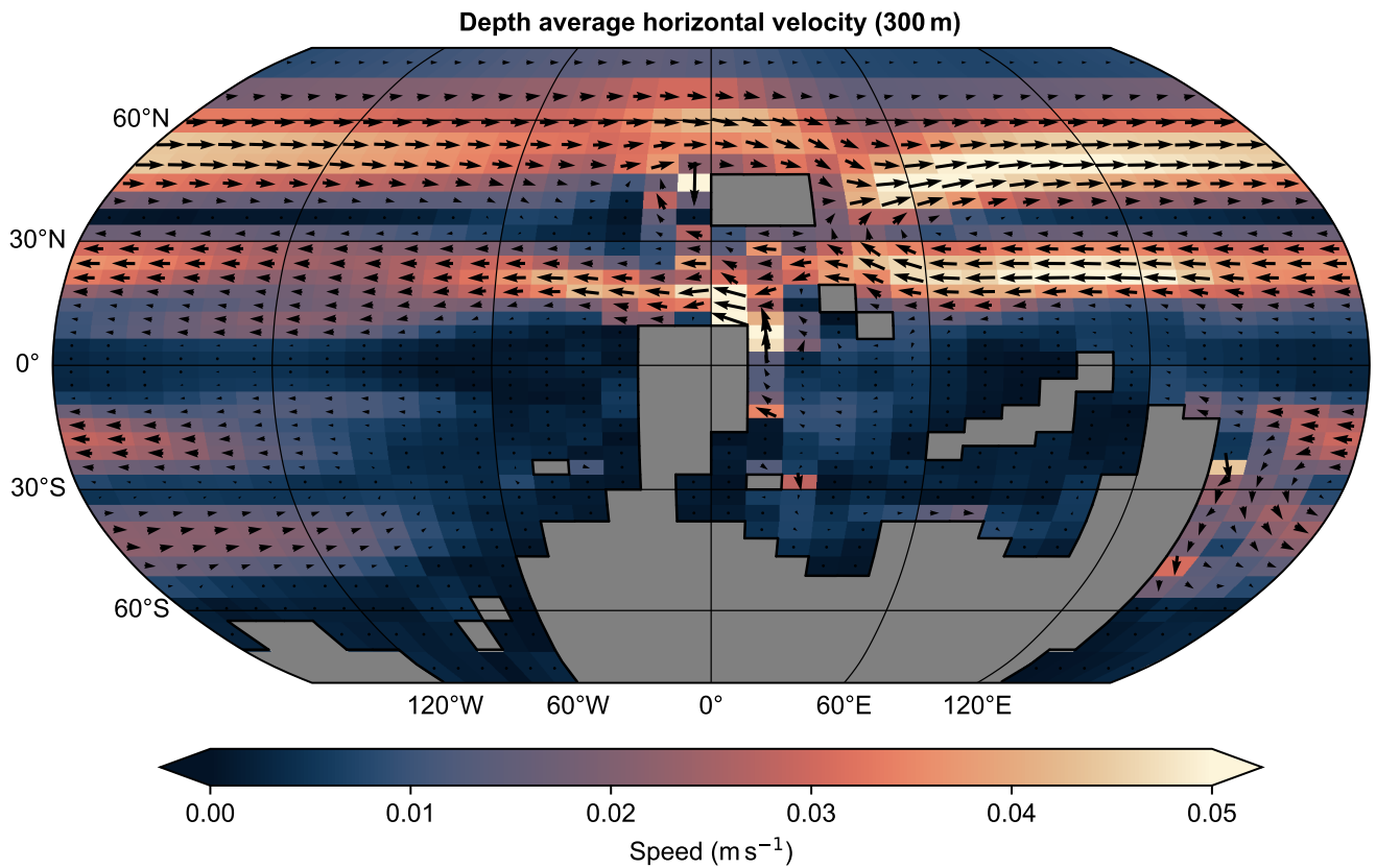
Figure 7. Surface ocean circulation. Mean horizontal ocean velocity ( \text{m}\cdot\text{s}^{-1} ) averaged over the upper 300 m. Arrow direction indicates flow orientation, while arrow length is proportional to velocity magnitude (also represented with background shading).
