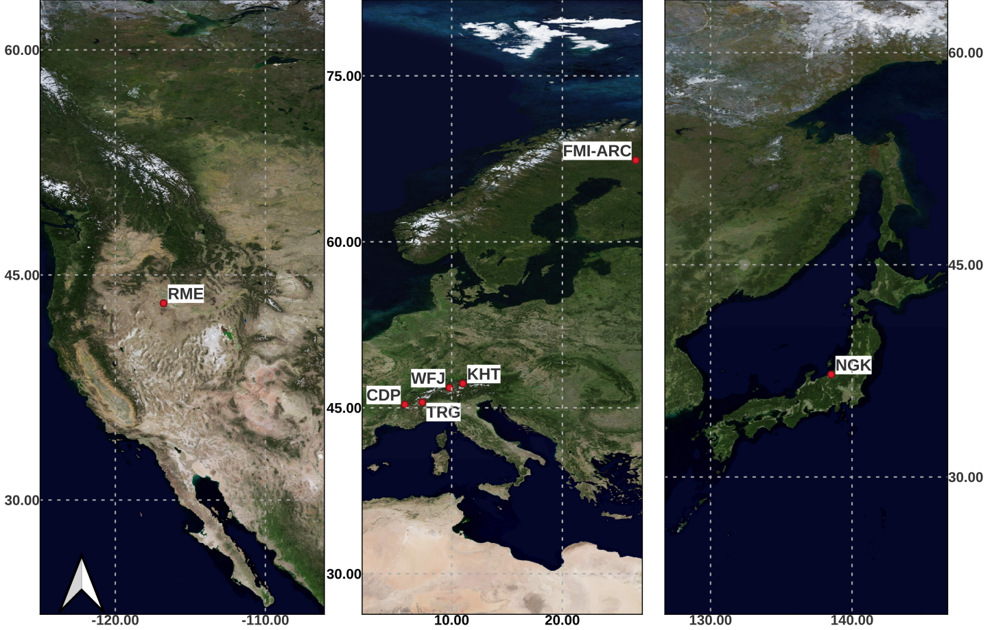
Figure 1. Geographical distribution of study sites used for snow modeling and data assimilation: (left) Reynolds Mountain East (RME) in the United States, (center) European sites including Col De Porte, Isère, France , Weissfluhjoch, Davos, Switzerland (WFJ), Torgnon, Aosta Valley, Italy (TRG), Kühtai, Tirol, Austria (KHT) FMI-ARC Sodankylä Geophysical Observatory, Finnish Lapland (FMI-ARC) in Finland, and (right) Nagaoka (NGK) Japan. Map created using the Free and Open Source QGIS.
