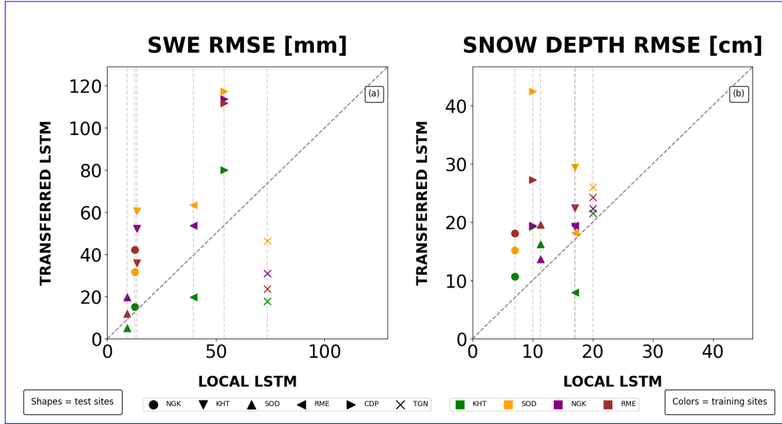
Figure 7. Spatial transferability of site-specific LSTMs for SWE and snow depth estimation. Panel (a) shows a comparison between the RMSE for SWE obtained by using each LSTM at the training site (x-axis) and the RMSE obtained when transferring the same LSTM to other sites (y-axis). Panel (b) shows the same information, but for snow depth. The bisectors in the two panels represent the one-to-one lines comparing the RMSE values for SWE and between the site-specific LSTM and the LSTM trained on a different site. The dotted lines in both panels serve as benchmarks, indicating the RMSE values achieved by the site-specific LSTM models. Colors represent training sites, while shapes correspond to the to sites where each LSTM was applied. The lowest granularity site, WFJ, is excluded.
