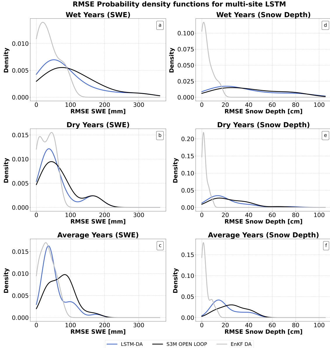
Figure 8. RMSE distribution for SWE and snow depth across water year types RMSE distribution for SWE on wet, dry and average years type (panels a,b,c) and snow depth (panels d,e,f) under varying water year types: wet, dry, and average conditions.
