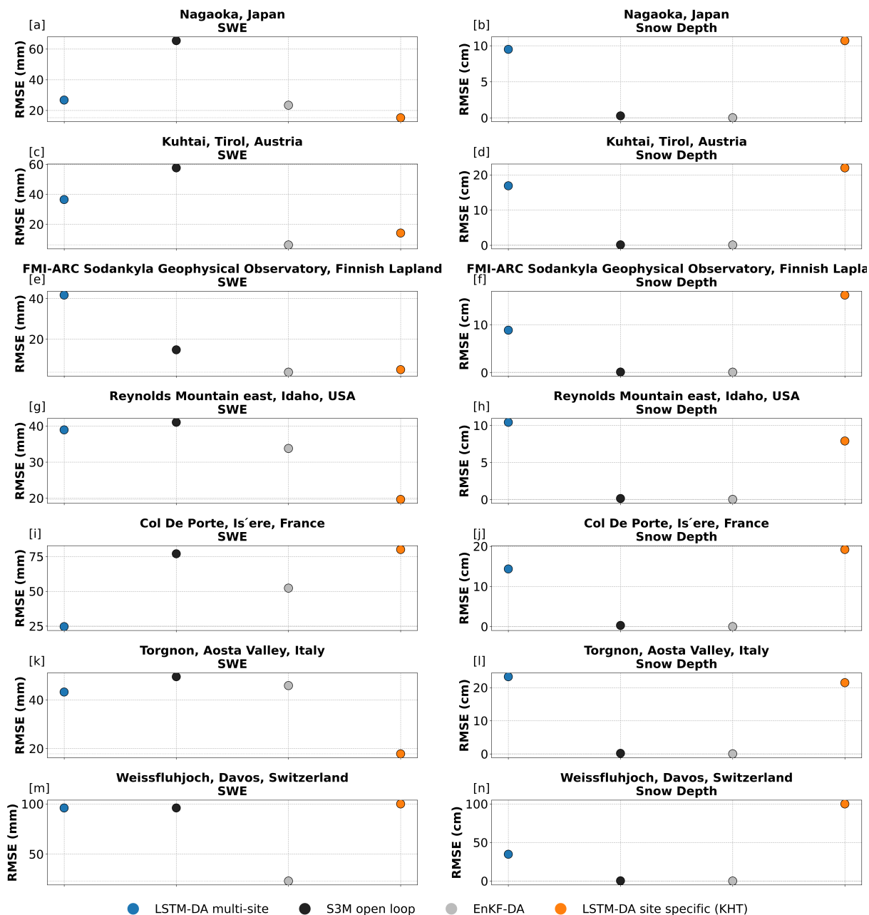
Figure 9. Comparison of RMSE for snow water equivalent (SWE, left column) and snow depth (right column) across multiple sites and methods. Results are shown for LSTM-DA multisite (blue), S3M open loop (black), EnKF-DA (grey), and LSTM-DA site-specific (KHT) (orange).
