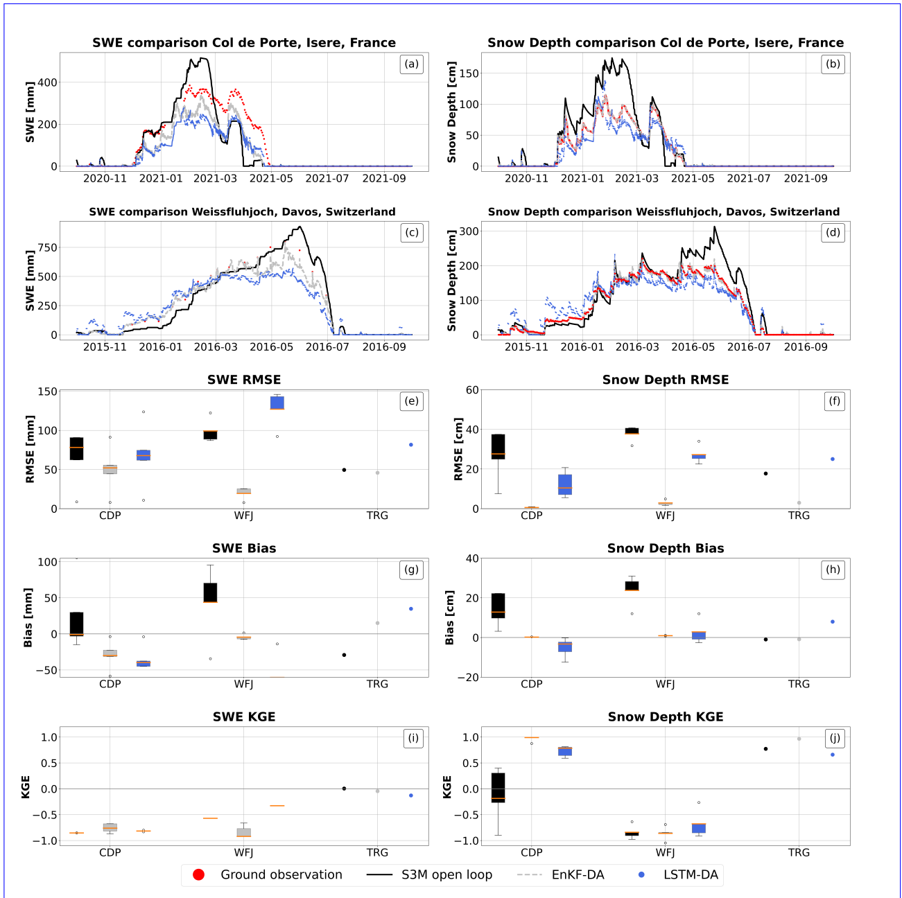
Figure 4. Results for sites with high data sparsity, site specific LSTM. Panel a,b,c,d: comparison between ground observation (red) of Snow Water Equivalent (top) and snow depth (bottom) and model estimates by S3M in open loop (black), using an Ensemble Kalman filter (grey), and using a Long Short Term Memory neural network (blue) in Col de Porte (row 1) and Weissfluhjoch (row 2). Panels e,f,g,h,i,j: box plots of RMSE, bias and KGE for SWE (panel e for RMSE, panel f for bias and panel i for KGE) and snow depth (panel g for RMSE, panel h for Bias and panel j for KGE); points represent sites with less than 3 years of validation data.
