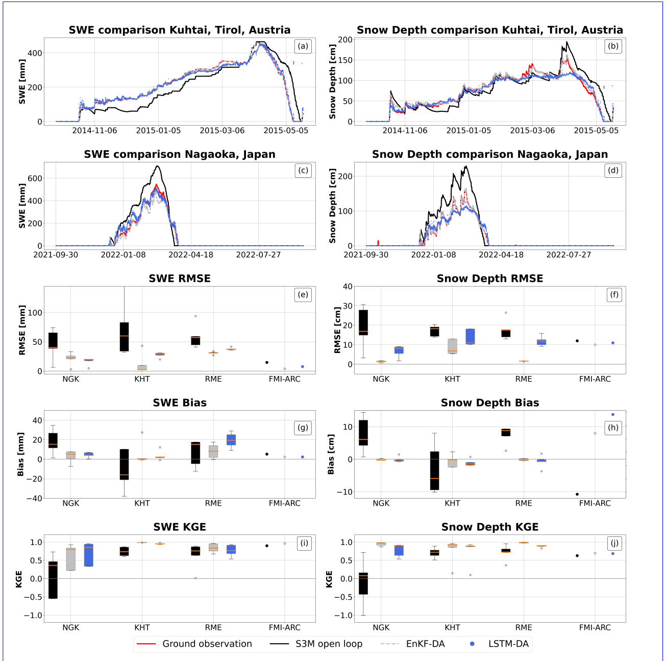
Figure 3. Results for sites with low data sparsity, site specific LSTM. Panels a,b,c,d: comparison between ground observation (red) of Snow Water Equivalent (top) and snow depth (bottom) and model estimates by S3M in the open loop (black), using an Ensemble Kalman filter (grey), and using a Long Short Term Memory neural network (blue) in Kuhtai (row 1) and Nagaoka (row 2). Panels e,f,g,h,i,j: box plots of RMSE, bias and KGE for SWE (pan.e for RMSE, panel f for bias and panel i for KGE) and snow depth (pan.g for RMSE, panel h for Bias and panel j for KGE); points represent sites with less than 3 years of validation data.
