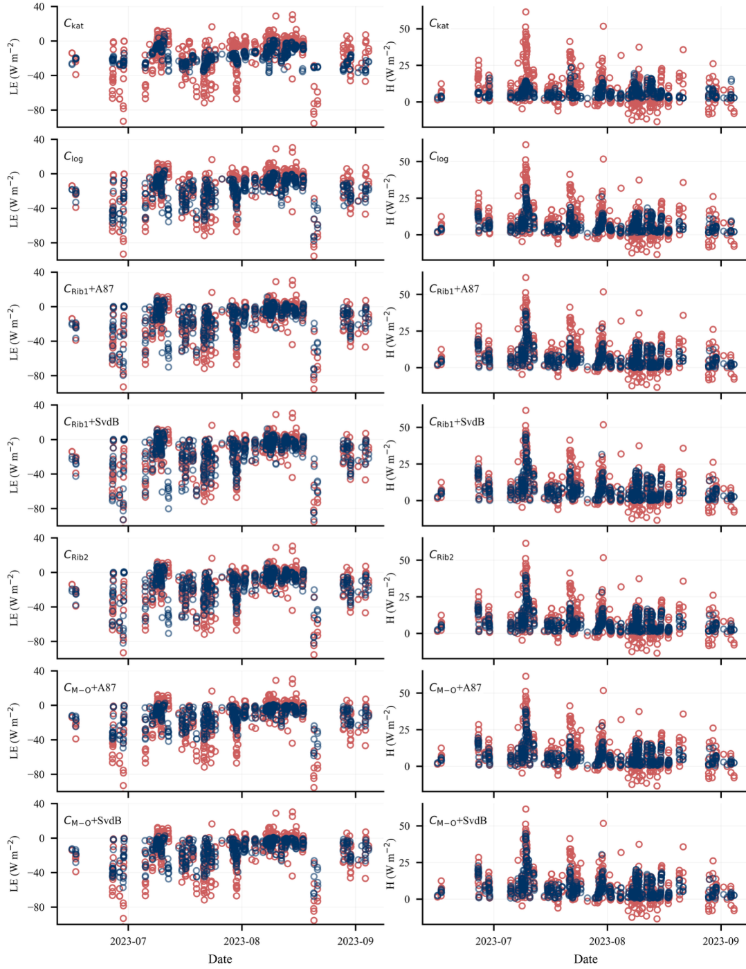
Figure 5: Time series of 30-min LE and H simulated by the five different schemes ( C_{kat} , C_{log} , C_{Rib1} , C_{Rib2} , and C_{M-O} ), compared with eddy covariance-derived values. The C_{Rib1} , C_{Rib2} , and C_{M-O} schemes were calculated by the observed aerodynamic roughness length ( z_{0m} = 1.2 \times 10^{-4} m), whereas C_{kat} and C_{log} were calculated using optimized parameters obtained by minimizing the differences between modeled and observed turbulent fluxes. Blue dots represent model simulations, and red dots denote observations.
