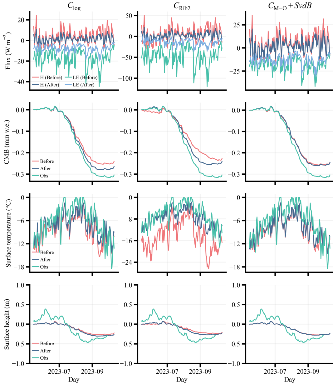
Figure 7: Time series of turbulent fluxes, cumulative mass balance (CMB), surface temperature, and surface height over the Dundee Glacier during the study period, based on original methods (before), recalibrated methods (after), and observations (obs).
