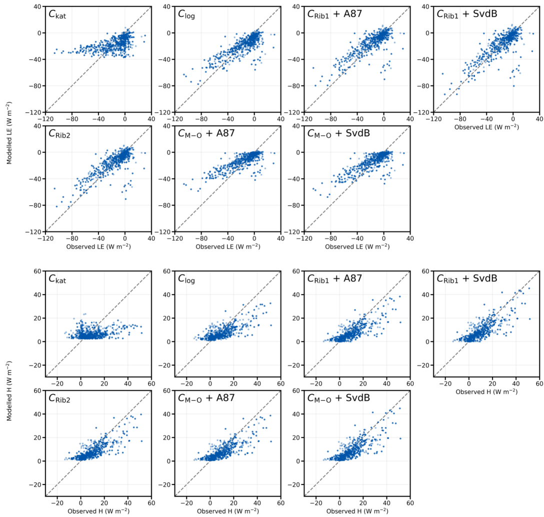
Figure 4: Comparison of 30-min observed (eddy-covariance-derived) and modeled H and LE according to the five turbulent flux methods.
