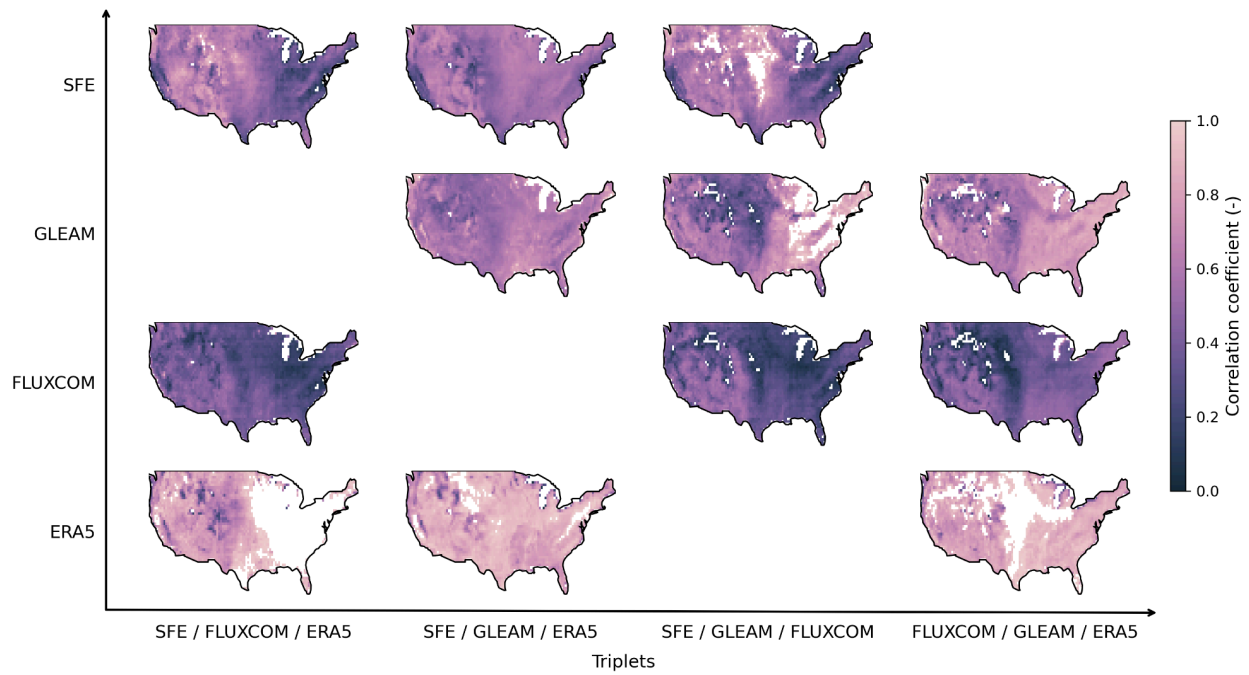
Figure S3. The correlation coefficient with the truth for each triplet (columns) and dataset (rows). White areas are those where the correlation coefficient is greater than one, indicating that the assumptions of triple collocation are not met.
