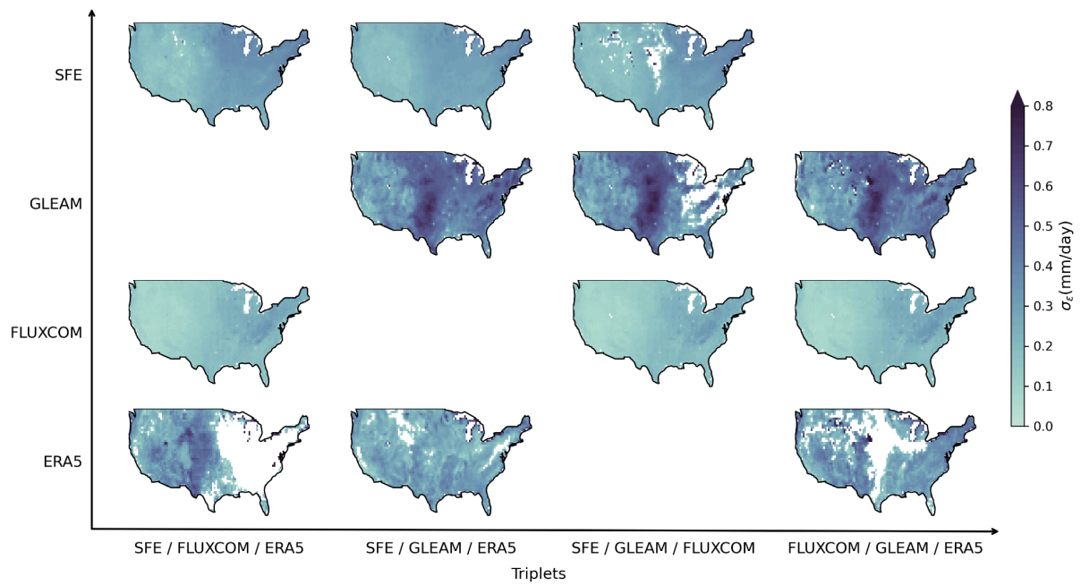
Figure S2. The random error standard deviation for each triplet (columns) and dataset (rows). White areas are those where the random error standard deviation can not be evaluated because of negative standard deviation, indicating that the assumptions of triple collocation are not met.
