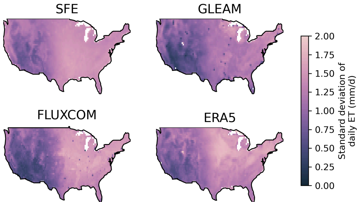
Figure S1. Standard deviation of daily ET from 1979-2016 for each dataset.
