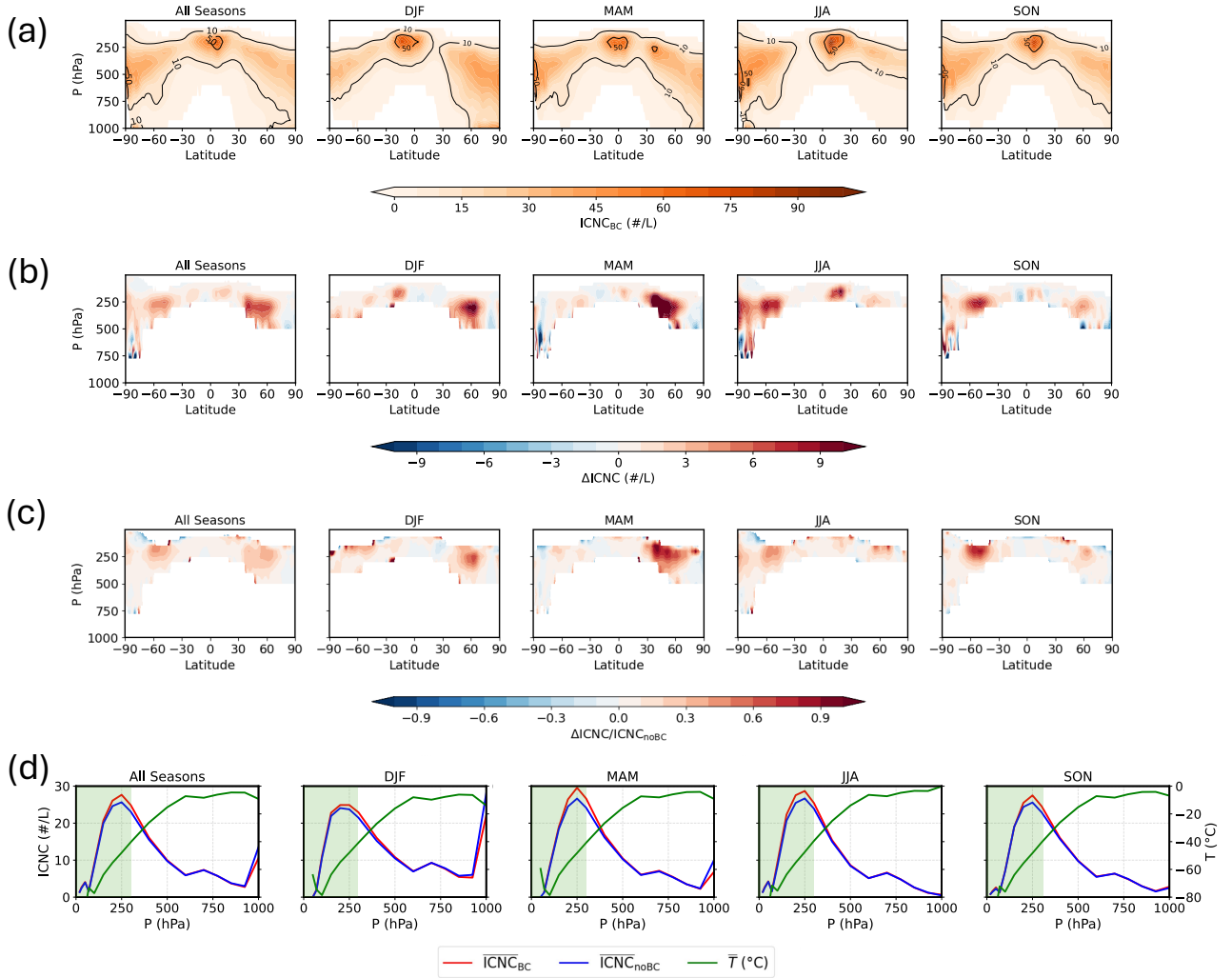
Figure 4. (a) Seasonal zonal mean of the ice crystal number concentration (ICNC; \# L^{-1} ) from GCM simulations with black carbon (BC) treated as ice-nucleating particles ( ICNC_{BC} ). The x-axis shows latitude, and the y-axis shows pressure (P; hPa). Each panel corresponds to a different season: annual average (All Seasons), December–January–February (DJF), March–April–May (MAM), June–July–August (JJA), and September–October–November (SON). (b) Seasonal zonal mean of the difference in ICNC ( \# L^{-1} ) between simulations with and without BC as INPs ( \Delta ICNC = ICNC_{BC} - ICNC_{noBC} ) at T < -40^{\circ}C . The x- and y-axes are the same as in panel (a). (c) Relative change in ICNC compared to simulations without BC as INPs, expressed as the ratio \Delta ICNC / ICNC_{noBC} at T < -40^{\circ}C . (d) Global-mean profiles of ice crystal number concentration (ICNC) and temperature, plotted using dual y-axes as a function of pressure. The left y-axis shows the globally averaged ICNC ( \# L^{-1} ) from GCM simulations with BC as INPs (BC, red solid line) and without BC as INPs (noBC, blue solid line). The right y-axis shows the corresponding global-mean temperature profile (green solid line). The shaded area indicates pressure levels where temperatures fall below -40^{\circ}C .
