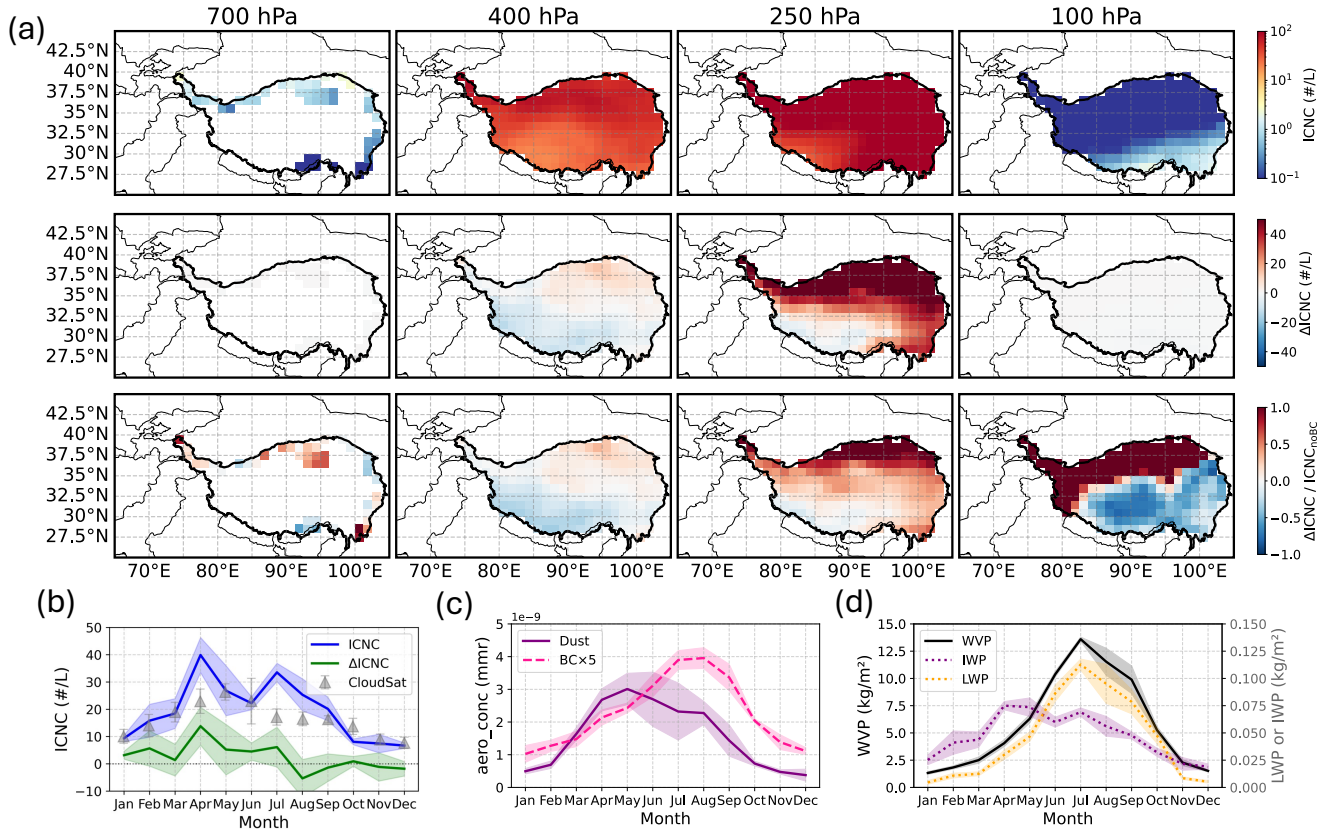
Figure 7. (a) Spatial distribution of ICNC during the spring (MAM) season over the Tibetan Plateau (TP). The first row shows the ICNC from the simulation including BC as INPs at various pressure levels. The second row displays the absolute difference in ICNC ( \Delta ICNC) between the simulations with and without BC as INPs. The third row illustrates the relative enhancement due to BC, calculated as \Delta ICNC / ICNC noBC . In all maps, the TP region is outlined by a thick black boundary. (b) Seasonal cycle of mean ICNC (blue line) and the mean change due to BC INPs ( \Delta ICNC, green line), spatially averaged over the TP and vertically averaged over altitudes where ice exists. The gray triangles show ICNC values from CloudSat averaged over 14 years reported by Chen et al. (2024). (c) Seasonal cycle of aerosol mass mixing ratios (mmr) averaged over the TP between 700 hPa and 100 hPa. The solid purple line shows the dust concentration, while the dashed pink line shows the BC concentration. Note that the BC concentration has been multiplied by a factor of 5 for improved visibility. (d) Seasonal cycle of column-integrated water path variables averaged over the TP. The plot shows the water vapor path (WVP, solid black line), ice water path (IWP, dotted purple line), and liquid water path (LWP, dotted orange line). Shaded regions in (b), (c) and (d) represent the standard deviation ( \pm 1\sigma ) for each variable.
