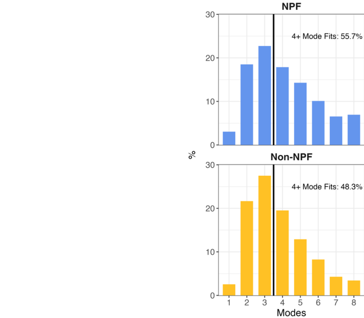
Figure 6 – Relative frequency of modes (%) necessary to successfully fit a PSD ( \text{NRMSE} \leq 10\% and \text{FVU} \leq 10\% ) on days where NPF was visually classified (top) or days where NPF was confirmed to not have occurred (bottom). Annotations indicate the percentage of data associated with 4 or more modes.
