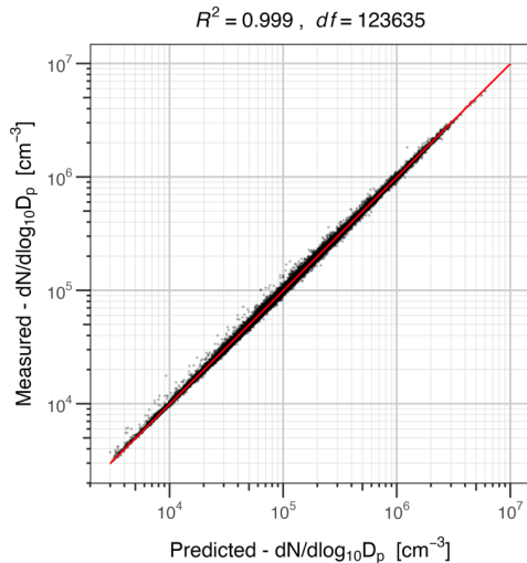
245 Figure 3 – Measured concentration vs predicted concentration dN/dlogD p for fittings above the accuracy thresholds of 0.1 (10%) FVU and NRMSE. Black dots represent prediction ratios for individual 10-minute averaged scans at SPL from 2010-01-14 to 2020-10-24. The red line is the simple linear regression of the predicted and measured particle concentration with coefficient of determination and degrees of freedom ( df ) listed in the title.
