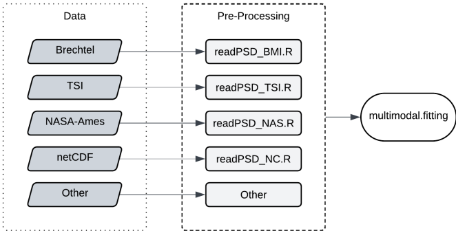
Figure 9– Flowchart summarizing the data formatting process to apply the methods described here to a variety of datasets.
