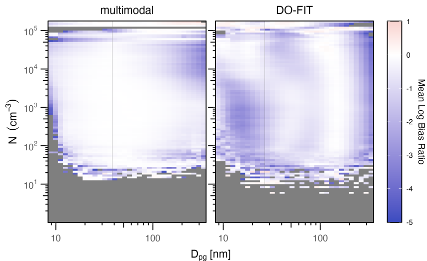
Figure 8 – Contour map of the magnitude in prediction error of the multimodal (left) and DO-FIT (right) PSD fitting algorithms. Red indicates overprediction whereas blue indicates underprediction, with the magnitude of error given in log scale (i.e. a value of -2 indicates the model underpredicts in this PSD region by 100x). Gray fill indicates regions where fitting failed.
