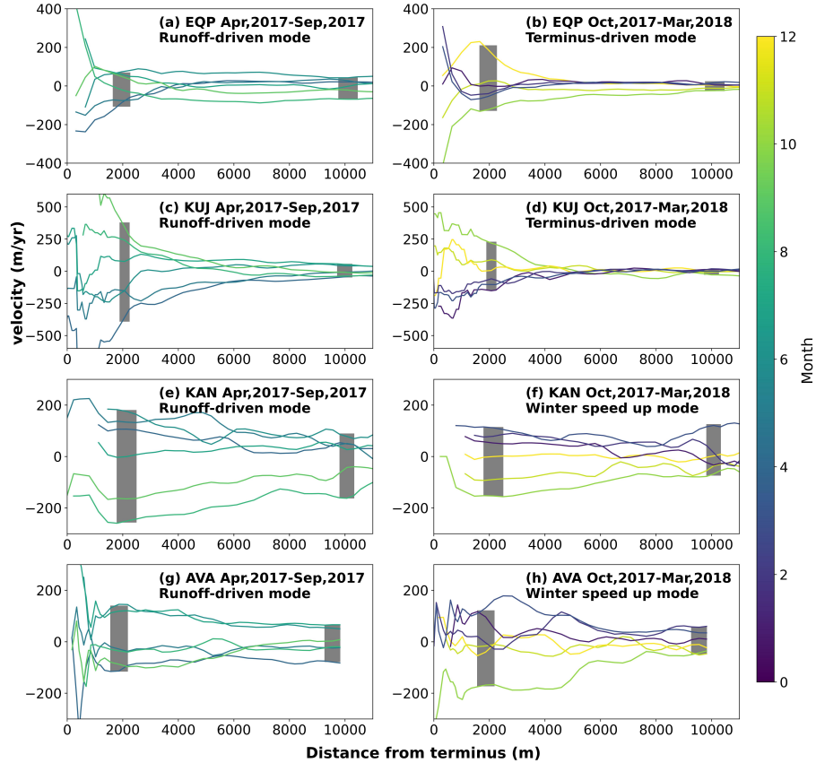
Figure 9. Velocity profiles over time for EQP, KUJ, KAN, and AVA. The average velocity profile has been subtracted for a better display of changes over time. The original velocity profiles are shown in Figure S8S7. The shaded areas indicate regions where we obtain velocity variations in the frontal (left) and upstream (right) sections. Left column (a, c, e, g) Velocity: Melt-season profiles of for EQP during the melt season. (ba) Velocity profiles of EQP after the melt season, during which velocity is primarily influenced by terminus changes. KUJ (c) Velocity profiles of KUJ during the melt season, KAN (e), and AVA (g). Right column (b, d, f, h) Velocity profiles of KUJ after the: Post-melt-season - profiles for EQP (eb) Velocity profile of KAN during melt season. KUJ (fd) Velocity profile of KAN after the melt season. (gf) Velocity profile of, and AVA during melt season. (h) Velocity profile of AVA after the melt season, when velocity is primarily influenced by terminus changes.
