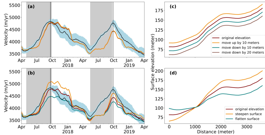
Figure 8. Experiment results for Kuj using the artificially modified surface elevations. The results of Panels (a) correspond to and (c) correspond to each other, and the results of as do (b) correspond to and (d). The blue shaded area represents observation uncertainties. Vertical black lines indicate the onset of the annual glacier retreat, and gray shaded vertical bars denote the melt season. In panel (d), the surface slope is altered by \pm 2\% within the 2 km frontal region.
