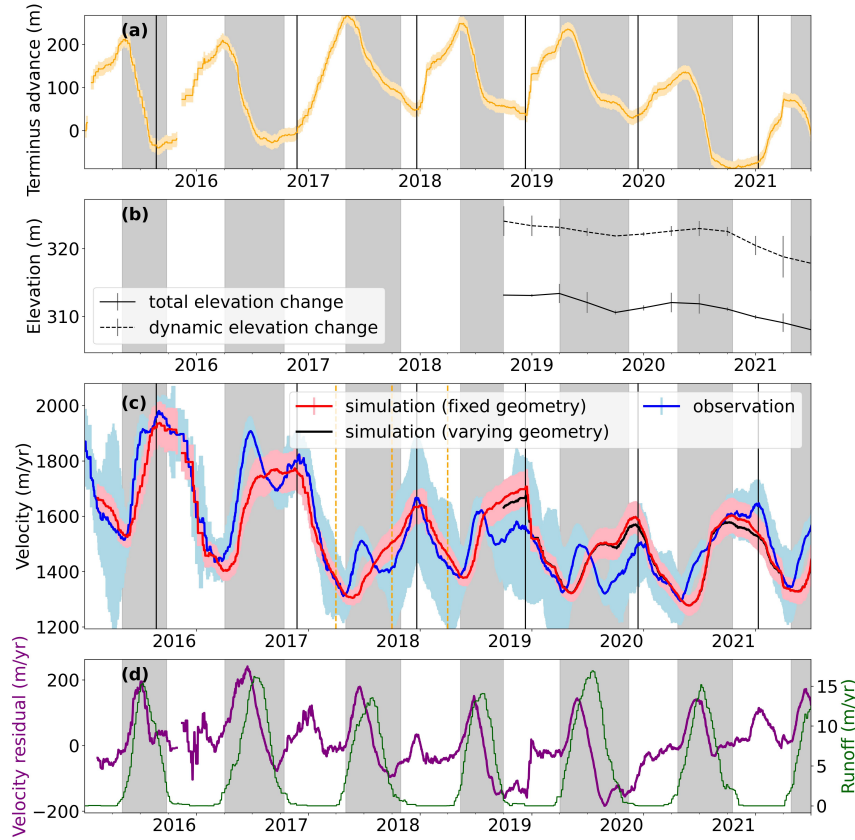
Figure 2. Time series for EQP. (a) Terminus position change time series from AutoTerm, with light yellow shading shows showing uncertainty. (b) Surface elevation from ICESat-2 data fusion. The dynamic elevation change is calculated by subtracting elevation change due to surface mass balance from total elevation change. (c) Observed and simulated velocity. Light blue and pink shading show the uncertainties of observations and simulations, respectively. (d) Velocity residual between observed and simulated velocity, along with the daily runoff from GSFC-FDMv1.2.1 ( values are per-unit-area runoff, in m/yr ). The In all panes, gray shaded-vertical bars in all panes indicate when mark melt seasons using the 1st percentile of each year's runoff is larger than 2 m/yr as the threshold. The vertical black lines mark the onset of annual glacier retreat. The orange dashed lines in (c) marks the two periods in Figure 9a and b, respectively.
