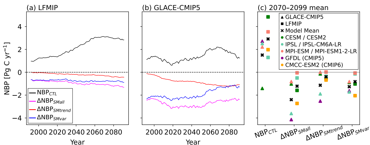
Figure 1. Comparison of the global evolution of NBP in (a) GLACE–CMIP5 and (b) LFMIP from 1991 to 2089 (smoothed with a 20 year centred rolling mean), including total NBP ( \text{NBP}_{CTL} , black), as well as the changes in NBP due to SM trend ( \Delta\text{NBP}_{\text{SMtrend}} , red), SM variability ( \Delta\text{NBP}_{\text{SMvar}} , blue) and the total SM effect ( \Delta\text{NBP}_{\text{SMall}} , pink), and (c) individual model projections of global mean NBP an and the respective SM–induced changes for the future period (2070–2099) for GLACE–CMIP5 (triangles) and LFMIP (squares). For panels (a) and (b) the colour-scheme-figure design was adapted-adopted from Green et al. (2019) to-facilitate-comparison-with-their-study .
