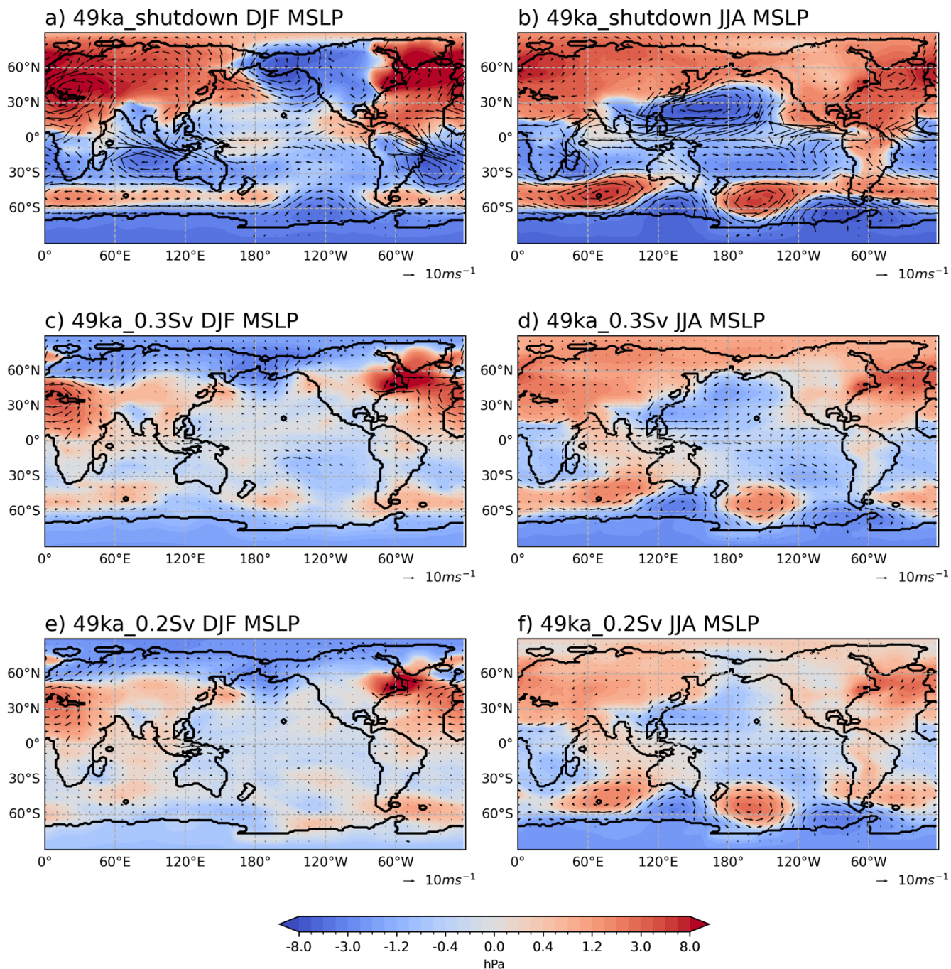
Figure 6: DJF (left column) and JJA (right column) MSLP anomalies (hPa) in each simulation relative to 49ka_control, with 850 hPa wind vector anomalies.
