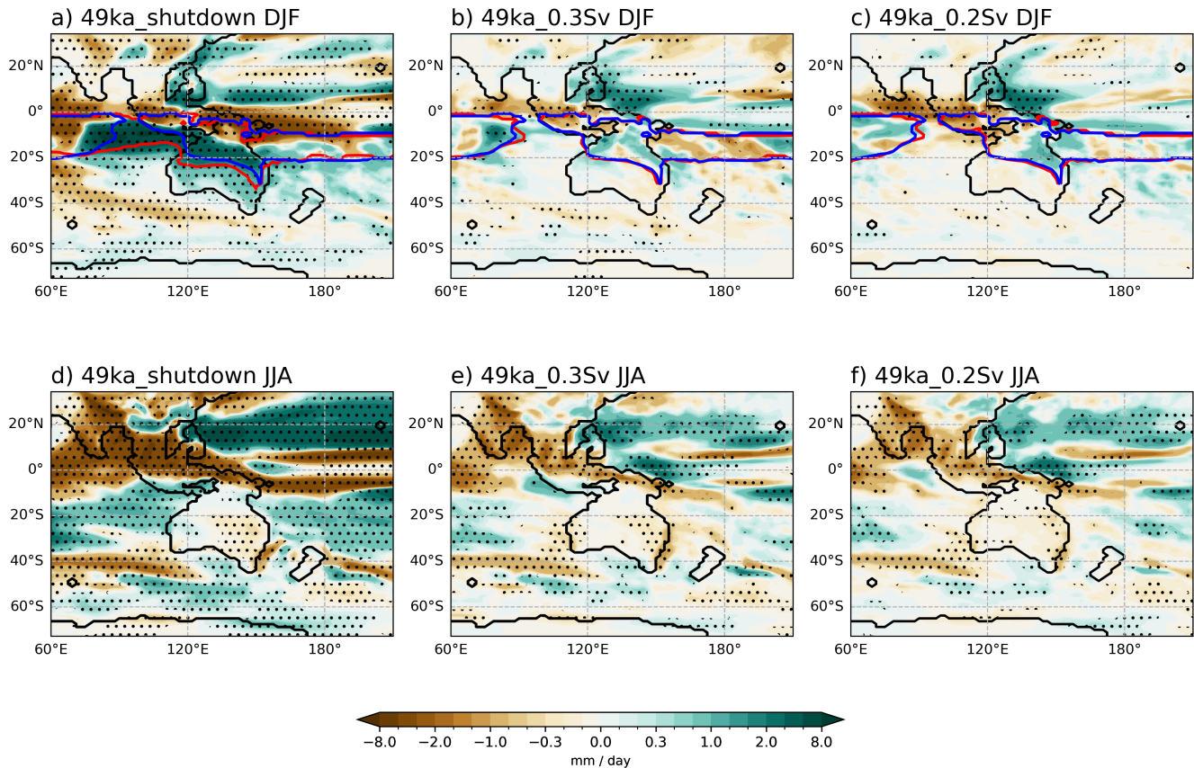
Figure 9: Australian DJF (top row) and JJA (bottom) precipitation anomalies in each simulation relative to 49ka_control (mm/day). The blue contours in DJF (a-c) represent the 49ka_control monsoon domains while the red contours indicate monsoon domains in each hosing experiments Stippling indicates areas with significant changes at the 95 % confidence level according to a Student's t-test.
