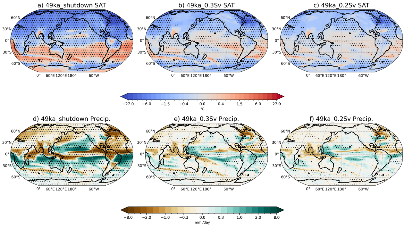
Figure 2: Annual (a)-(c) Surface Air Temperature (SAT; in °C) and (d)-(f) precipitation (in mm/day) anomalies relative to 49ka_control in each simulation. Stippling indicates statically significant differences from the control at the 95 % confidence 230 level according to the Student's t-test.
