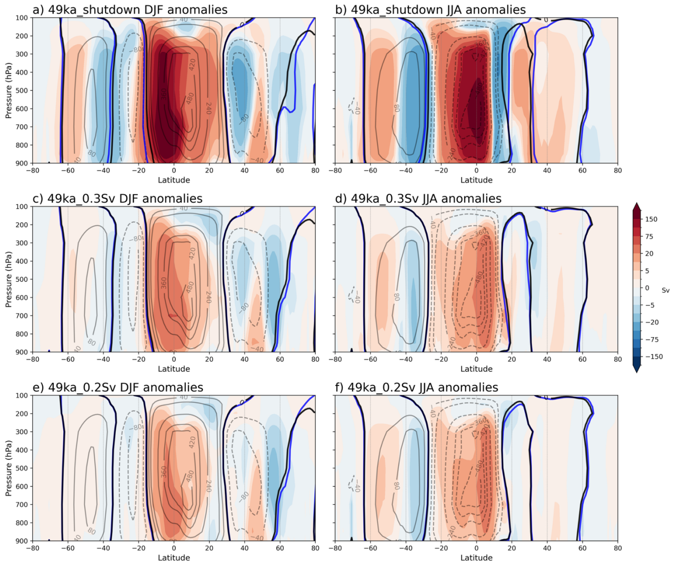
Figure 4: DJF and JJA 49ka_shutdown (a, b), 49ka_0.3Sv (c, d), and 49ka_0.2Sv (e, f) minus 49ka_control atmospheric mass streamfunction anomalies (Sv, shading). Black contours (solid=positive; dashed=negative) are 49ka_control absolute streamfunction values. The thick black and blue lines represent the zero contour in 49ka_control and each freshwater hosing experiments, respectively.
