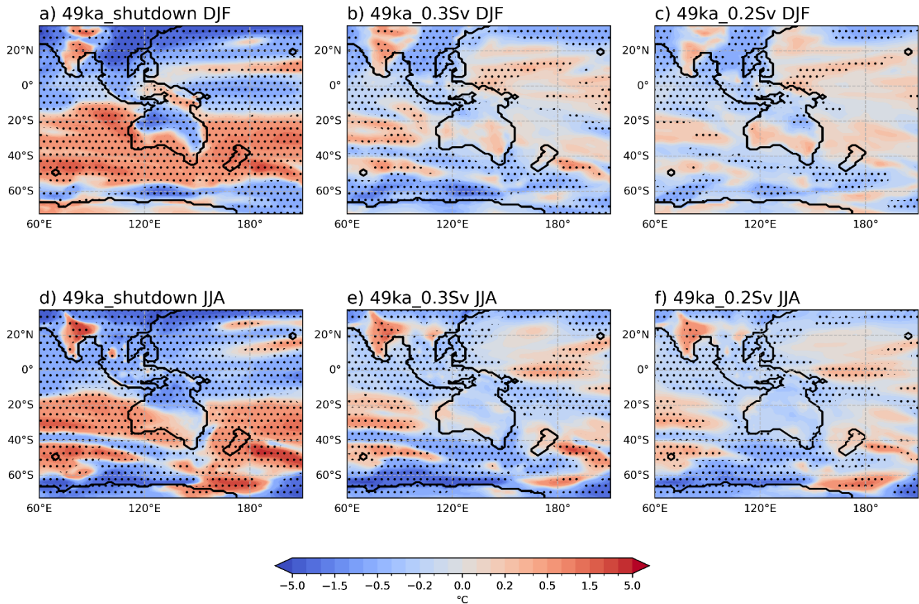
Figure 8: Australian annual DJF (top row) and JJA (bottom) surface air temperature (SAT; in °C) anomalies in each simulation relative to 49ka_control. Stippling indicates areas with significant changes at the 95 % confidence level according to a Student's t-test.
