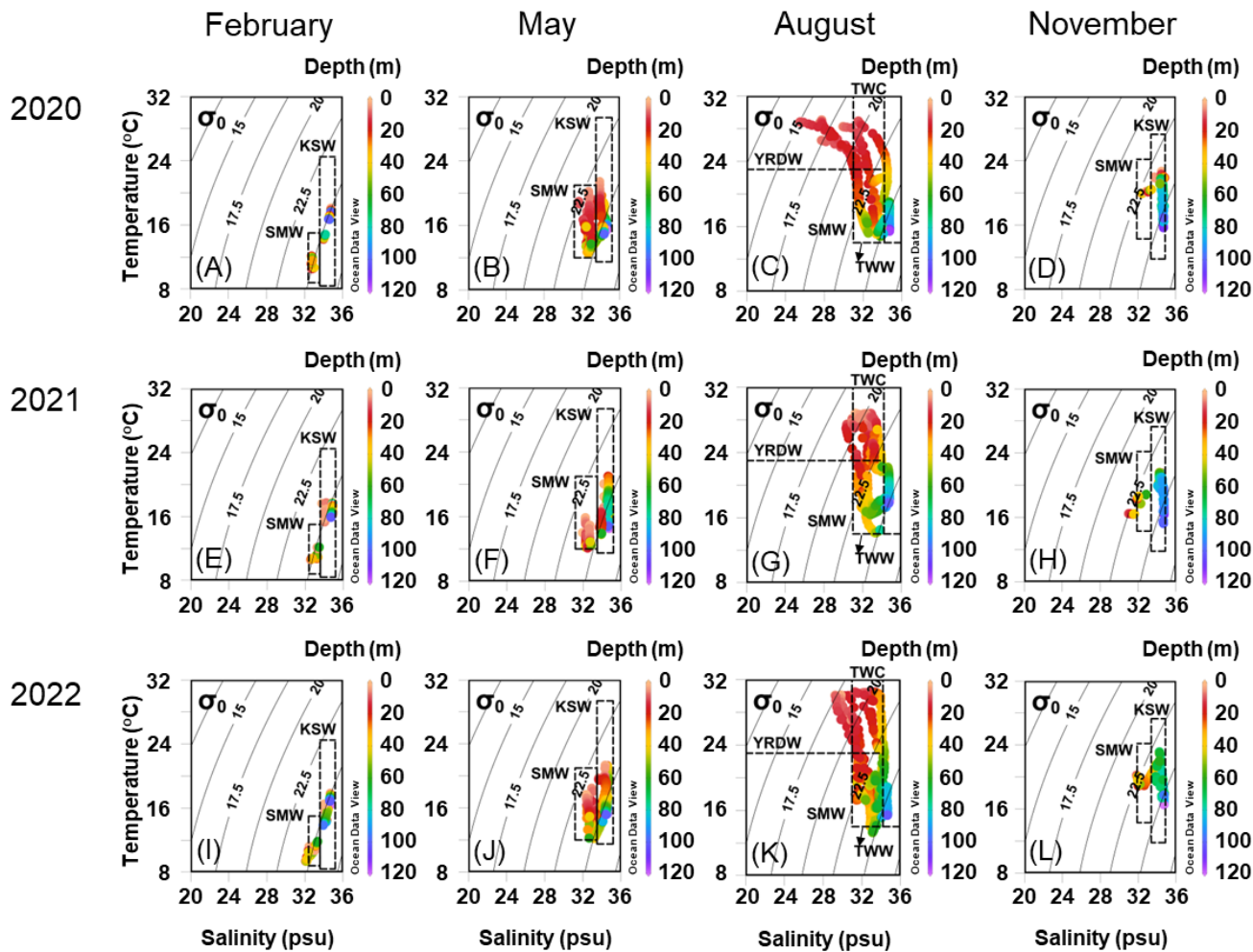
Figure 2. Seasonal T-S diagrams of the East China Sea (ECS) in 2020 (A, B, C, D), 2021 (E, F, G, H), and 2022 (I, J, K, L). The dashed box indicates the defined water masses in this study observed in the northern ECS (Gong et al., 1996; Hur et al., 1999; Kim and Youn, 2023). Grey contour lines represent the sigma-t. The color bar indicates the depth of the water column.
