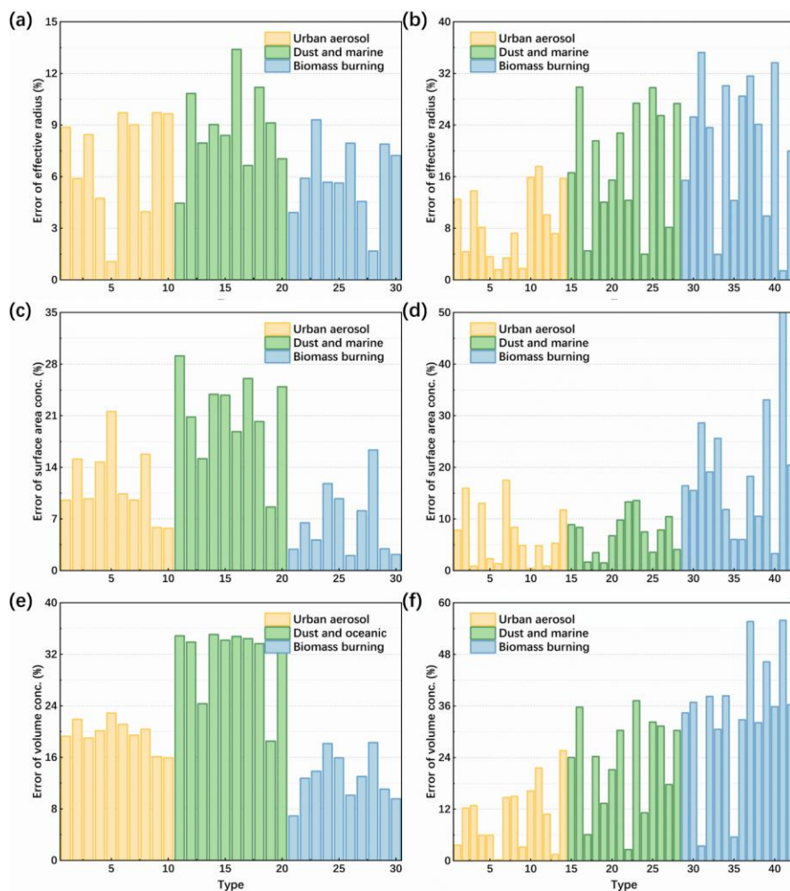
230 Figure 2: AMP error statistics for simulations of three aerosol modals. The statistical data for the unimodal distribution are presented on the left side, and the bimodal distribution are shown on the right.
