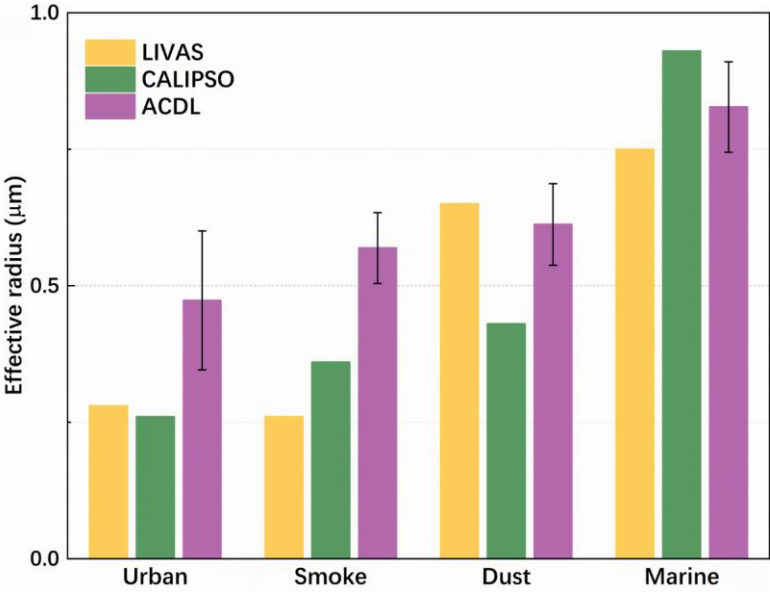
Figure 1012: Comparison of ACDL inversion effective radius results with CALIPSO and LIVAS
