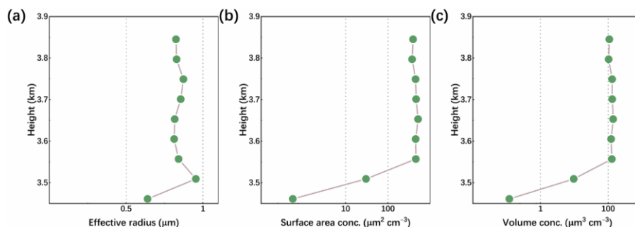
Figure 911: Marine aerosol AMP inversion from ACDL data products
