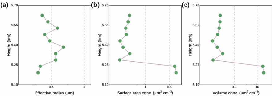
Figure 68: Urban aerosol AMP inversion from ACDL data products
