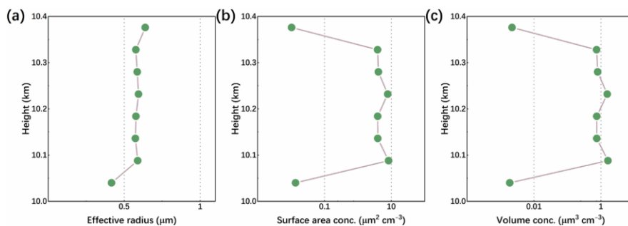
Figure 79: Smoke aerosol AMP inversion from ACDL data products
