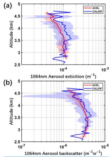
Figure 6: Vertical profiles of aerosol backscattering and extinction coefficients at 1064 nm from ACDL and CALIPSO, along with their corresponding standard deviation estimates. The vertical profiles aerosol backscattering and extinction coefficients at 532 nm, 1064 nm, 1572 nm obtained from ACDL, along with their corresponding standard deviation estimates, are shown in Figure 7, which selected from ACDL measurements on March 1st, 2023. Figure 7(a) shows the retrieved aerosol extinction coefficients profile, and Figure 7(b) shows the backscatter coefficients profile. The blue curves represent the 1064 nm signals, and the red curves correspond to 1572 nm. The shaded areas denote the estimated standard deviations. It can be observed that the uncertainty associated with 1572 nm signal is slightly larger than that of the 1064 nm signal. This behaviour is physically explainable, the design of the
