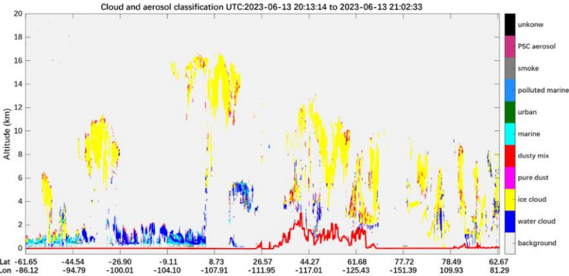
Figure 5: Cloud and aerosol classification on 13 June 2023, 20:13-21:02, retrieved from ACDL. The red line denotes the surface elevation
