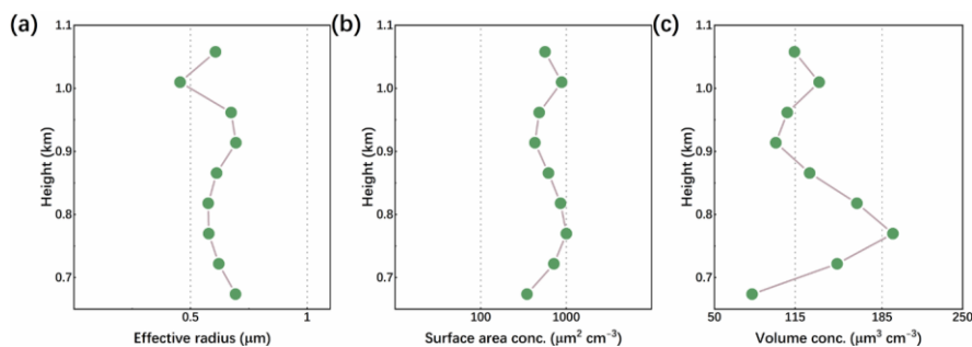
Figure 810: Dust aerosol AMP inversion from ACDL data products
