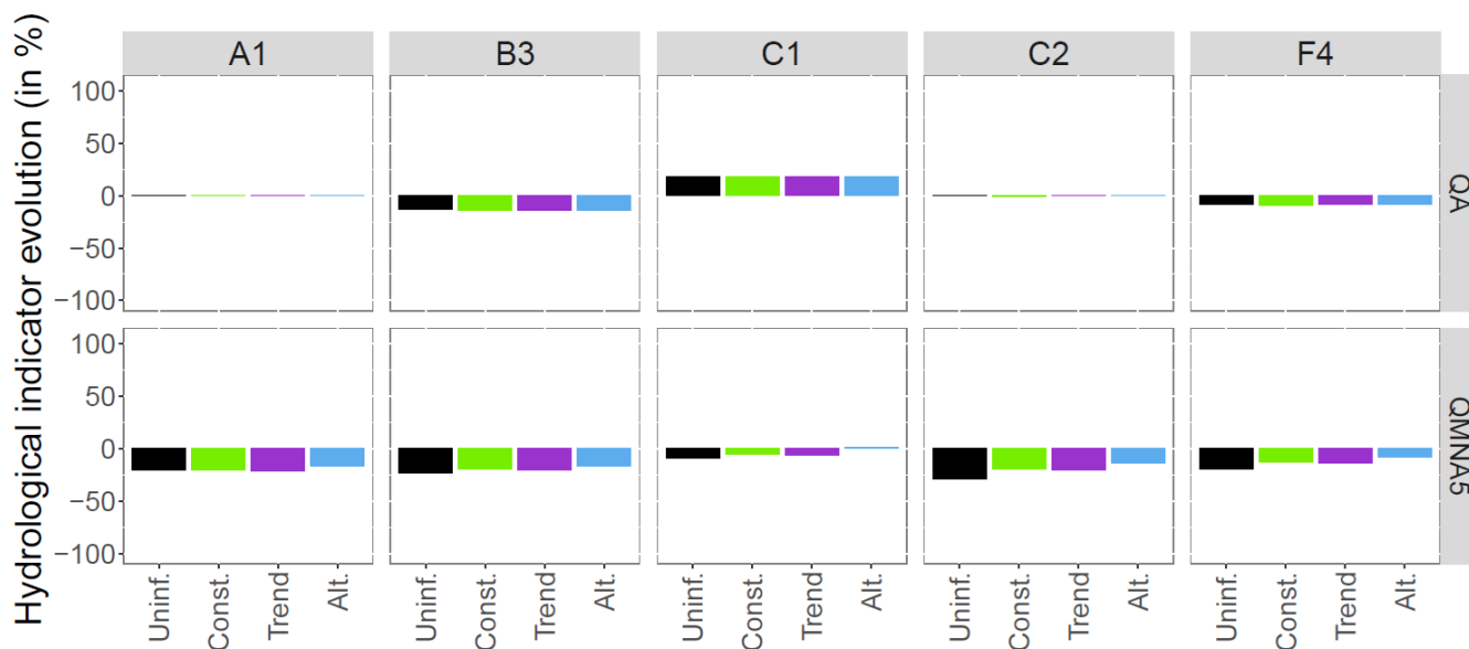
485 Figure 8: Evolution of mean flows (QA, row 1) and low flows (QMNA5, row 2) indicators at the catchment outlet (Sèvre Nantaise at Nantes) for the uninfluenced simulation and the three future scenarios for the five climate projections (in columns). The evolutions are calculated from 2056-2085 to 1976-2005.
