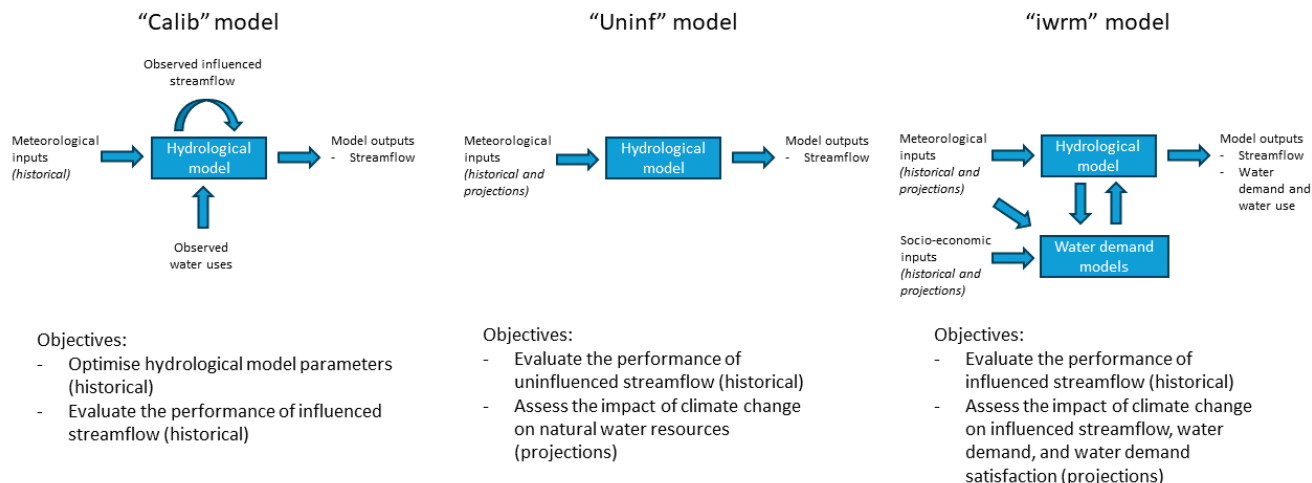
335 Figure 3: The three conceptual hydrological modelling frameworks integrating, or not, water uses, and their objectives. The hydrological model is only calibrated in the “Calib” version.
