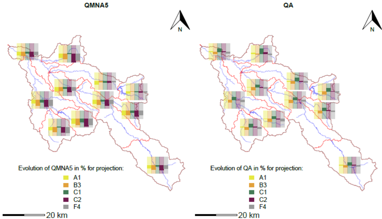
Figure 6: Evolution in percentage of the hydrological indicators obtained with the “Unif” model under five climate projections for the 11 Management Units of the Sèvre Nantaise for 2056-2085 compared to 1976-2005. The shaded bars indicate the -50 to +50 % range. QA stands for mean flows and QMNA5 is an indicator of low flows.
