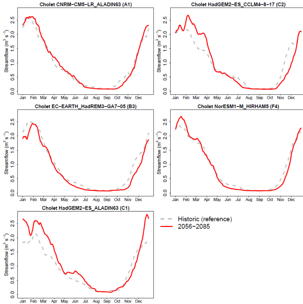
1055 Figure F1: Interannual streamflow regime for the projected uninfluenced streamflow for the Cholet gauge station (downstream of the Ribou-Verdon dams) for 2056-2085 for the five climate projections.
