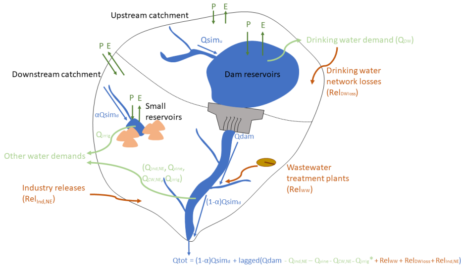
330 Figure 2: Schematic of the functioning of the integrated hydrological model. Two catchments are shown: the upstream catchment includes a dam reservoir large dam (corresponding to MU1 and MU3 in the Sèvre Nantaise catchment), while the downstream catchment does not include any dam reservoir large dam (corresponding to all other MUs). Small reservoirs and the related water demands, as well as wastewater treatment plants, can be present in both cases but are shown in the downstream catchment only for graphical purposes. The dam reservoir outflow (Q dam ) is determined according to the management rules given in Table D1 and is delayed towards the catchment outlet proportionally to the hydraulic distance from the dam to the outlet. The simulated streamflow in the downstream catchment (Q sim,d ) is given by a GR6J model. Part of this (α) is captured by small reservoirs. The total streamflow at the outlet is the sum of all streamflows (from the dam, the downstream catchment and the water releases) minus the water withdrawals, which are delayed according to the hydraulic distances between the withdrawal and release points. All other fluxes and notations are detailed in Appendix D. Natural fluxes are in dark green, streamflow is in blue, water withdrawals in light green, and water releases in dark orange.
