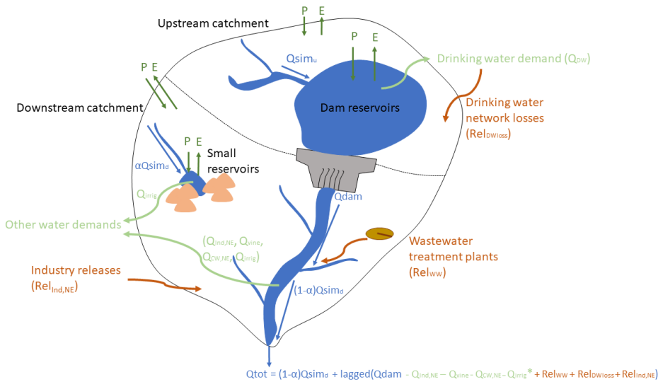
380 Figure 2: Schematic of the functioning of the integrated hydrological model. Two catchments are shown: the upstream catchment includes a dam reservoir (corresponding to MU1 and MU3 in the Sèvre Nantaise catchment), while the downstream catchment does not include any dam reservoir (corresponding to all other MUs). Small reservoirs and the related water demands, as well as wastewater treatment plants, can be present in both cases but are shown in the downstream catchment only for graphical purposes. The dam reservoir outflow ( Q_{dam} ) is determined according to the management rules given in Table D1 and is lagged towards the
